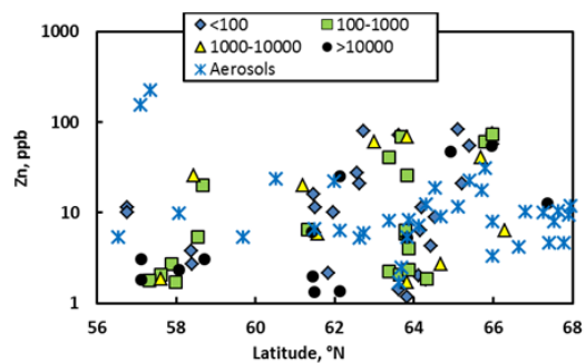
Figure 2. Winter snow soluble concentration of Zn (blue asterisk) compared with actual concentrations in rivers during spring flood (May-June) of different size of the watershed (diamonds, squares, triangles and circles correspond to < 100, 100-1000, 1000-10,000 and > 10,000 km 2 surface area, respectively) in western Siberia along the latitudinal gradient (Shevchenko et al., 2016 in preparation).
