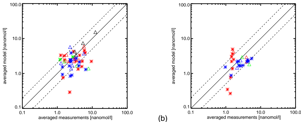
Fig. 2. Scatter plot of simulated and measured annual mean DMS sea surface concentrations averaged over the biogeochemical provinces defined by Longhurst et al. (1995). Provinces for the Atlantic Ocean in red, the Indian Ocean in green, the Pacific Ocean in blue, and the Southern Ocean in black. Provinces in the Southern Hemisphere are indicated by a triangle, in the Northern Hemisphere by an asterisk. Exact values are listed in Tables 5 and 6. (a) Measurements from the Kettle and Andreae (2000) database. (b) Measurements obtained from http://saga.pmel.noaa.gov/dms/ , excluding the measurements of the Kettle and Andreae (2000) database. The solid line indicates the 1:1 ratio, the dashed lines the 1:2 and 2:1 ratios. Units are nmol/l.
