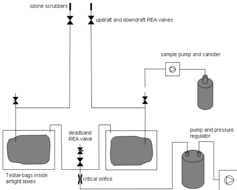
Fig. 1. A block diagram of the REA flow system used in this study.
