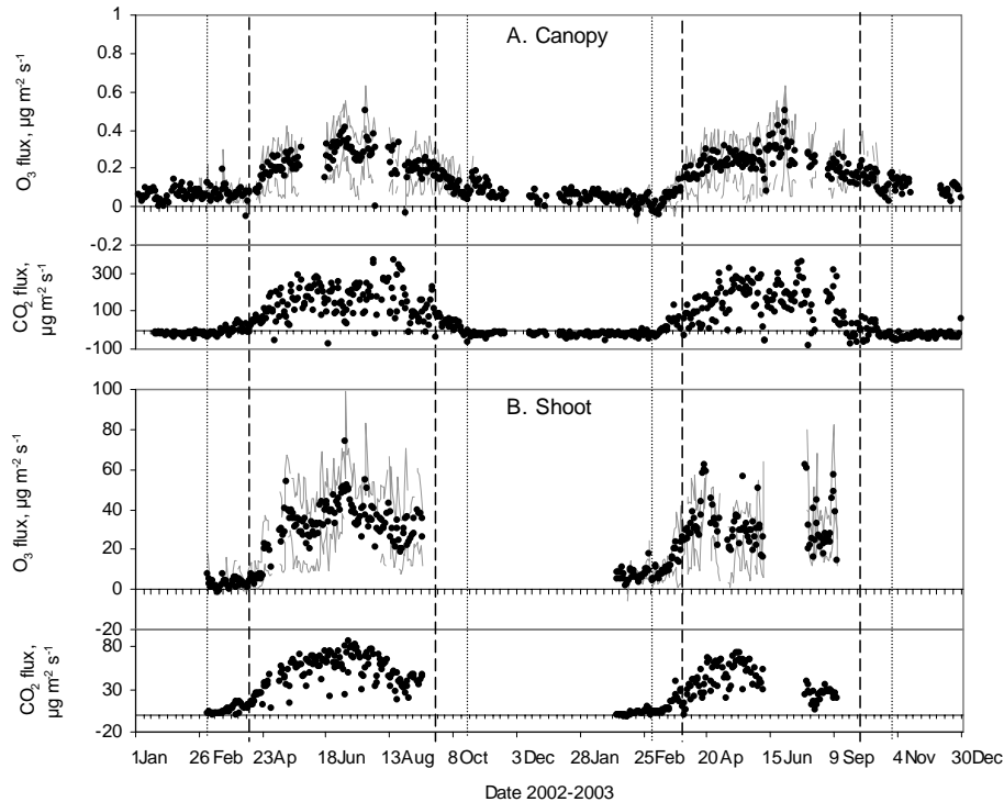
Fig. 1. Annual patterns of daily O_3 and CO_2 fluxes in SMEAR II during 2002–2003 measured at (A) canopy and (B) shoot scale. Positive values denote uptake by the plant. Black dots are values of: whole-day averaged fluxes. Lines are day and night averaged O_3 flux (upper and lower line, respectively). The flux of CO_2 relates to the intensity of forest activity. Seasons are also marked by the vertical lines (dashed —): the start and end of the thermal growing season, daily mean temperature >5^\circ\text{C} ; and (dotted ...): the start and end of the thermal winter, daily mean temperature <0^\circ\text{C} .
