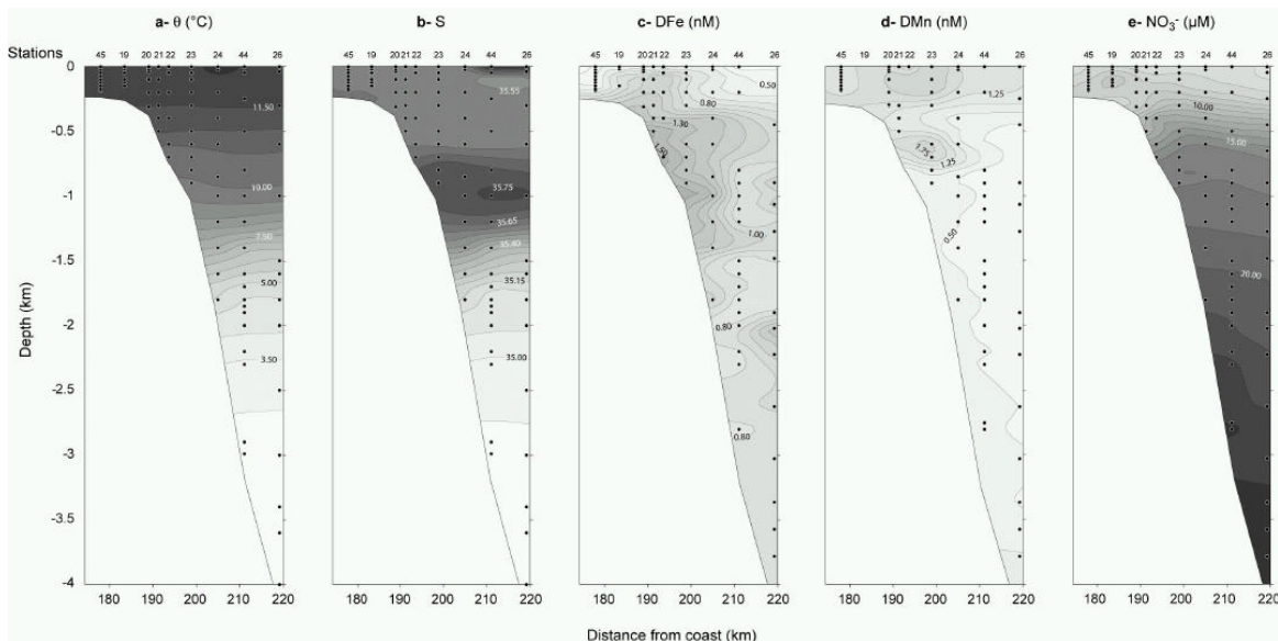
Fig. 6. Two dimensional distributions of potential temperature ( \Theta , a ), salinity (S, b ), concentrations of DFe, DMn ( d ), and \text{NO}_3^- ( e ) over the slope.
