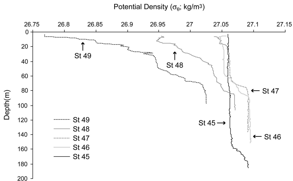
Fig. 3. Potential density ( \sigma_{\theta} , \text{kg/m}^3 ) profiles for St 49, 48, 47, 46, and 45.
