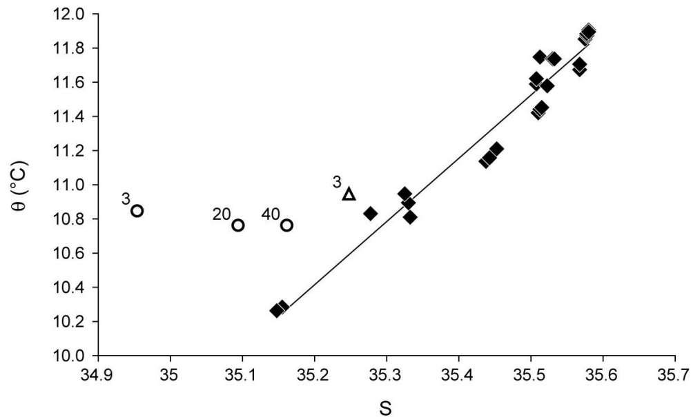
Fig. 4. Salinity-potential temperature ( \Theta -S) diagram for the plateau ( \Theta=3.72S-120.58 , R^2=0.96 , standard deviation of slope 0.16, standard deviation of intercept: 0.10, opened triangle: 3 m for St 48, opened circles: 3, 20 and 40 m for St 49).
