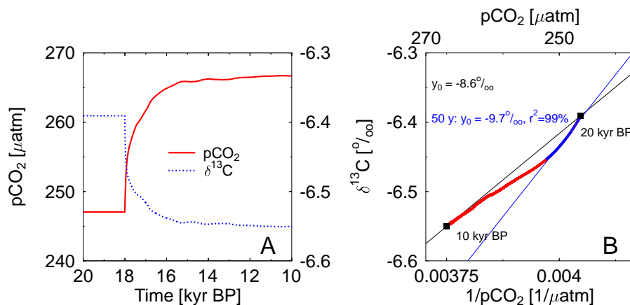
Fig. 10. Effects of iron fertilisation in the Southern Ocean on atmospheric carbon records with scenario taken from Köhler et al. (2005a) (A: pCO 2 , δ 13 C; B: Keeling plot). Blue dots and regression in (B) over the first 50 years during pCO 2 rise only.
