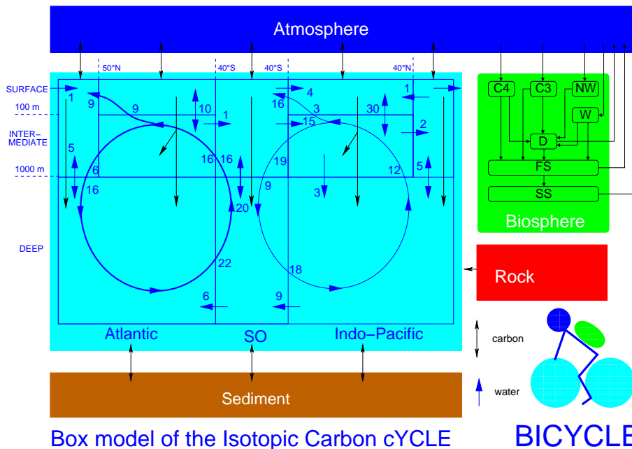
Fig. 4. A sketch of the BICYCLE model including boundary conditions and preindustrial ocean circulation fluxes (in \text{Sv}=10^6 \text{ m}^2 \text{ s}^{-1} ) in the ocean module. The globally averaged terrestrial biosphere distinguishes ground vegetation following different photosynthetic pathways (C4, C3), non-woody (NW), and woody (W) parts of trees, and soil compartments (D, FS, SS) with different turnover times.
