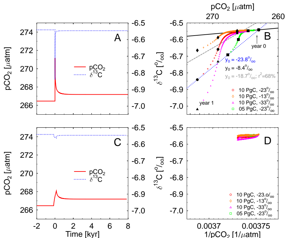
Fig. 6. Effect of a pulse of instantaneous release (within one year) of terrestrial carbon with an isotopic signature of \delta^{13}\text{C} = -23\text{‰} (left: \text{pCO}_2 , \delta^{13}\text{C} ; right: Keeling plot). Different carbon release amplitudes (5, 10 PgC) and different \delta^{13}\text{C} signatures ( -13\text{‰} , -23\text{‰} , -33\text{‰} ) are tested. The regression functions seen in (B) are for the three different regression models for the 10 PgC/ -23\text{‰} scenario (red circles). Model 1: year 0 and year 1 (short dash); model 2: year 0 and year 8000 (solid); model 3: regression through 375 years (long dash). Large black markers mark the years 0, 1, 10, 100 in each record. Bottom: Same as above but now the data are smoothed with a 300 yr running mean.
