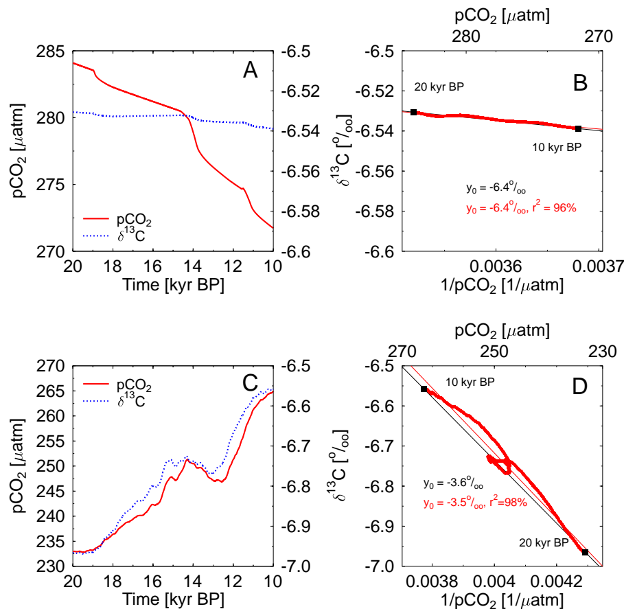
Fig. 13. Simulated effects of sea level rise (top) and ocean temperature change (bottom) as used in Köhler et al. (2005a) (left: \text{pCO}_2 , \delta^{13}\text{C} ; right: Keeling plot). Regression of the prior/after analysis (black) and over the whole period (red) are shown.
