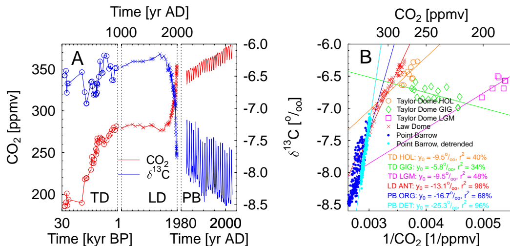
Fig. 1. A compilation of data from Point Barrow (PB), the Law Dome (LD), and the Taylor Dome (TD) ice cores ( A : CO 2 , δ 13 C; B : Keeling plot). Monthly resolved data (1982–2002) from Point Barrow (Keeling and Whorf, 2005; Keeling et al., 2005). Only times where data in both CO 2 and δ 13 C were available are considered here. For the Keeling plot approach the original data (PB ORG) and detrended time series (PB DET) are plotted and analysed. Data from firn and ice at Law Dome cover the last millenium (Francey et al., 1999; Trudinger et al., 1999) which includes the anthropogenic rise in CO 2 (LD ANT). Data from the Taylor Dome ice core of the last 30 kyr include the glacial/interglacial transition during Termination I (Smith et al., 1999) with the age model of Brook et al. (2000). Taylor Dome data are split into the Holocene (TD HOL), the glacial/interglacial transition (TD GIG), and the LGM (TD LGM).
