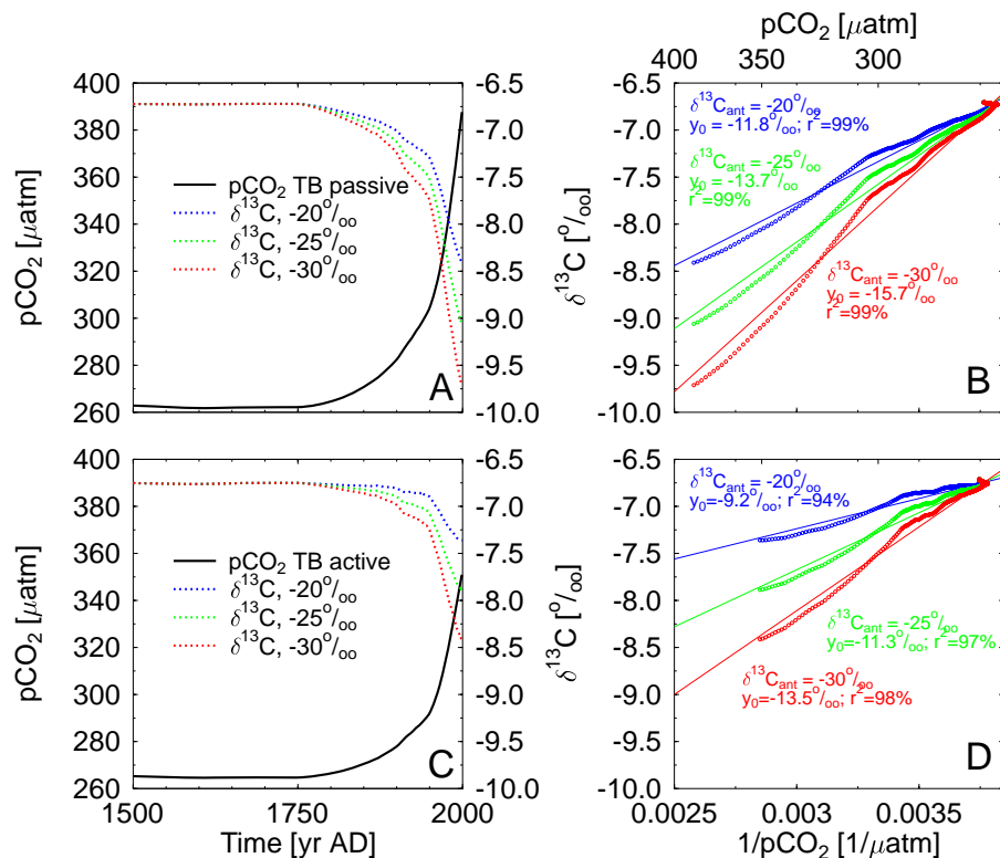
Fig. 5. Reconstructions of the rise in p\text{CO}_2 during the last 500 years with BICYCLE (left: p\text{CO}_2 , \delta^{13}\text{C} ; right: Keeling plot). Anthropogenic fluxes were used as plotted in Fig. 2. Two different settings are tested, one with passive terrestrial biosphere TB (top), meaning that carbon storage in the land reservoirs was kept constant, and one with active terrestrial biosphere (bottom), in which a rise in the internal calculated p\text{CO}_2 is enhancing terrestrial carbon uptake via its fertilisation effect. Different simulations with different isotopic signatures of the anthropogenic emission ( -20\text{‰} , -25\text{‰} , -30\text{‰} ).
