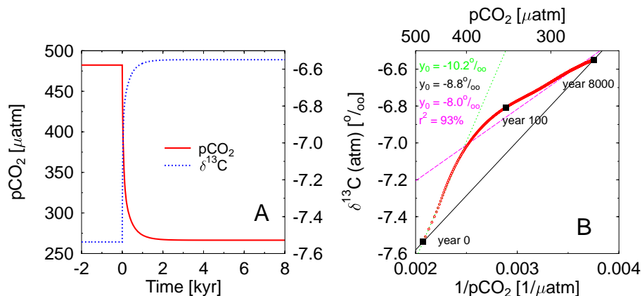
Fig. 9. Switching from an abiotic to a biotic ocean at t=0 kyr ( A: \text{pCO}_2 , \delta^{13}\text{C} ; B: Keeling plot). Different regression models in (B): model 1 (first year only) in green; model 2 (prior/after) in black; model 3 (equilibration time) in magenta.
