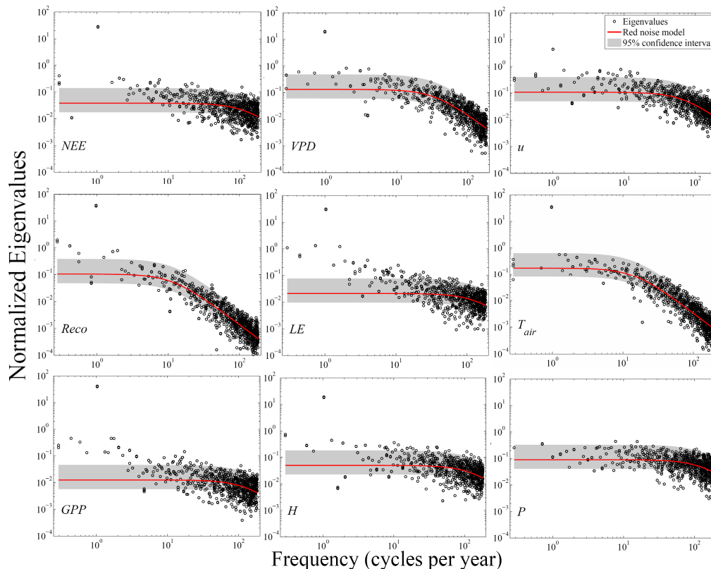
Fig. 1. The eigenspectra of the observed time series for NEE , R_{eco} , GPP , VPD , LE , H , u , T , and P . The dots represent the dominant frequencies of the time series at the respective normalized eigenvalue. The latter is equivalent to the amount of allocated variance. The red lines show the fitted red noise model. The gray areas are the corresponding 95% significance intervals.
