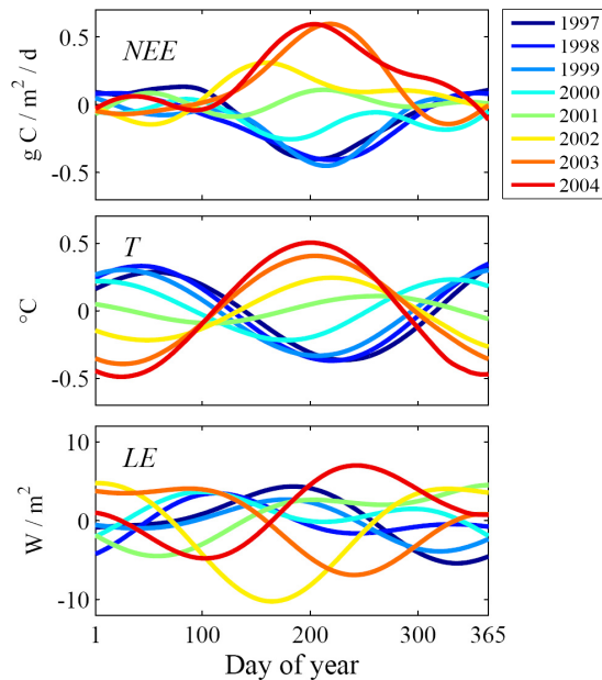
Fig. 6. The deviations of the estimated mean reference component of NEE , T and LE , based on the joint reconstruction of the annual and interannual components.
