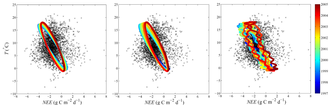
Fig. 3. The cross relationship of the partly reconstructed NEE and T time series. From left to right: The first panel shows the pure annual components of both variables where the colour code permits tracing the temporal evolution. The black crosses show the respective red noise components. The centre panel time series reconstruction is based on the annual and interannual components. The right panel shows a reconstruction, where also the significant intraannual components were considered.
