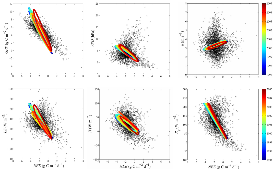
Fig. 4. The cross relationships of the major variables with NEE . Black crosses show the respective red noise components. The colour coded reconstructed components comprise the annual and interannual components of the respective variables, where the colour code permits tracing the temporal evolution.
