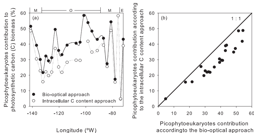
Fig. 9. Picophytoeukaryotes contribution to the photosynthetic carbon biomass as derived from c_{euk} 's contribution to c_{veg} by applying Eq. (5) (bio-optical method) and as obtained using intracellular carbon contents in Table 3 to estimate picophytoplankton carbon biomass (a). When comparing the results obtained using both approaches, it can clearly be seen that the contributions estimated using the intracellular carbon (C) content approach are lower than those estimated using the bio-optical approach, with almost all data points being below the 1-to-1 line relating both estimates (b).
