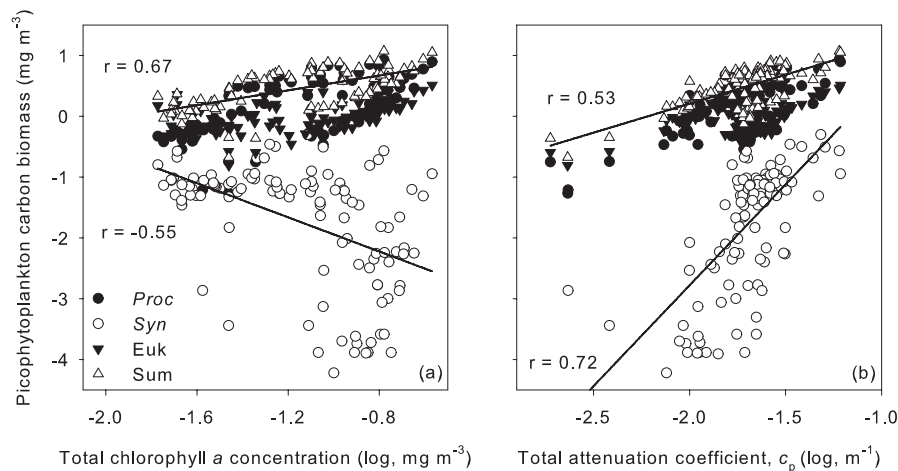
Fig. 8. Log-log relationships for Prochlorococcus ( Proc ), Synechococcus ( Syn ), picophytoeukaryotes ( Euk ), Proc + Euk ( Sum ) carbon biomass (mg m -3 ) with total chlorophyll a concentration in mg m -3 (a) and total particulate attenuation coefficient in m -1 (b). Only data from Stations 3 to 15 and GYR and between the surface and 1.5 Ze are included (see Sect. 2.2). Correlation coefficients ( r ) were calculated for Sum and Syn carbon biomass with Tchl a (a) and c p (b).
