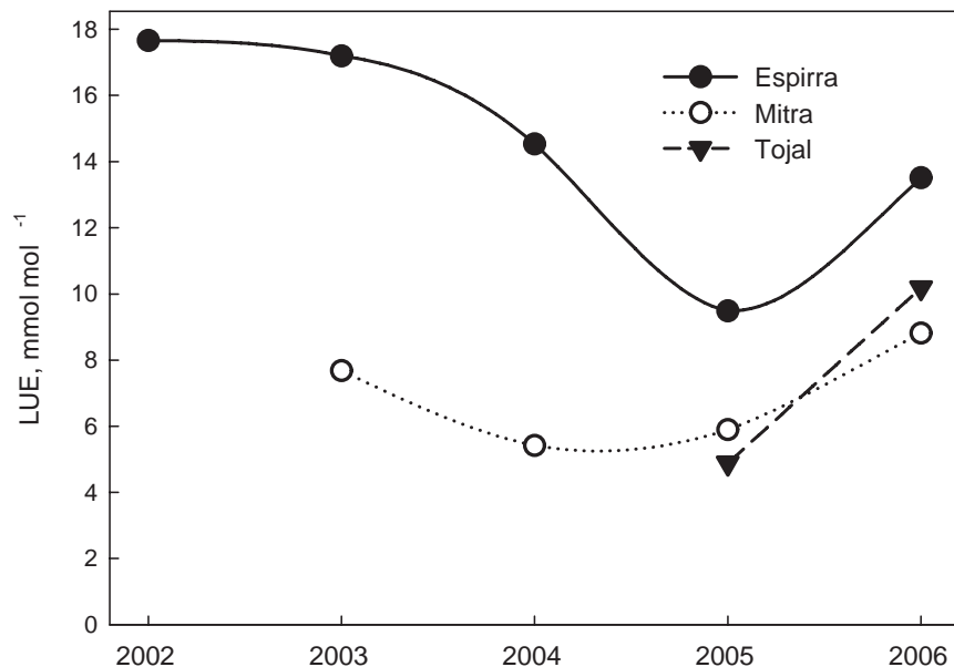
Fig. 7. Gross ecological light use efficiency, ( LUE_{ecol} , \text{mmol mol}^{-1} ) expressed in monthly averages for the three experimental sites (Espirra – eucalypt plantation; Mitra – oak savannah; and Tojal – grassland) during the extended experimental period (2002–2006).
