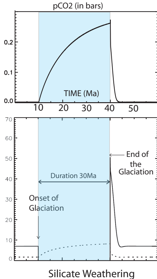
Fig. 4. CO 2 evolution as a function of the snowball earth duration and silicate weathering flux (in 10 12 mol/yr) respectively due to continental weathering (black line) and seafloor weathering (dash line). The blue bland represents the glaciation duration.
