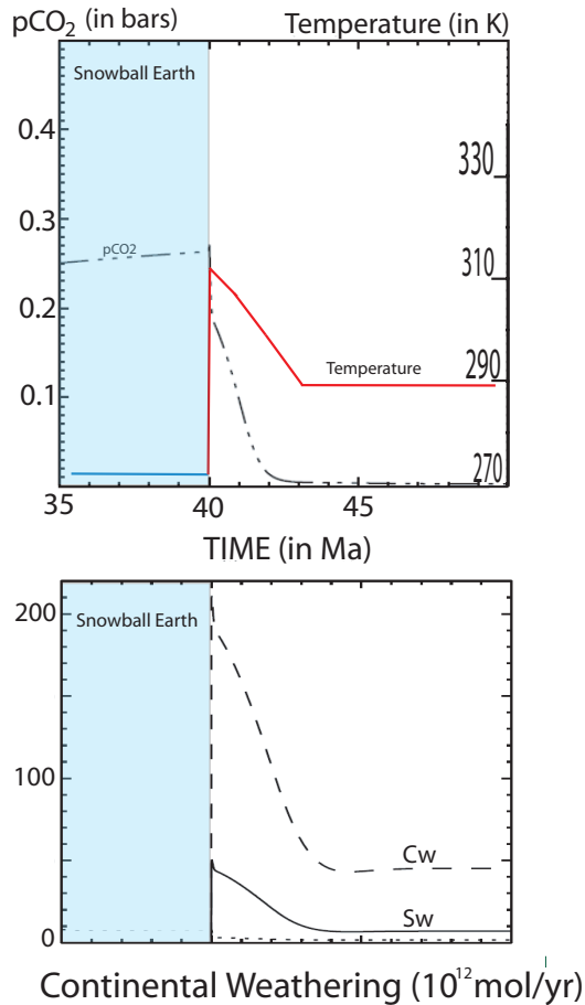
Fig. 7. Temperature, pCO 2 and weathering flux in the aftermath of the glaciation. The blue shaded represents the glaciation duration. Cw is for Carbonate Weathering rate (dash line) and Sw for Silicate Weathering (black line).
