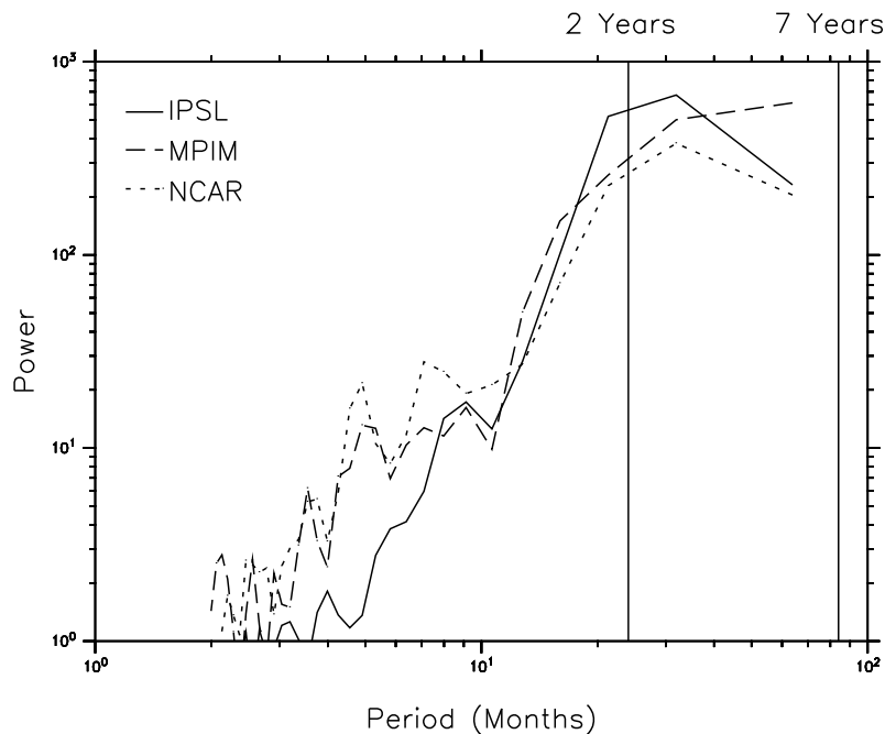
Fig. 3. Maximum entropy power spectra of modelled sea surface temperatures (SST) averaged over the Nino3 Box ( 150^{\circ} W– 90^{\circ} W, 5^{\circ} S– 5^{\circ} N). The vertical lines correspond to periods of two and seven years, respectively, corresponding to the typical range of ENSO frequency.
