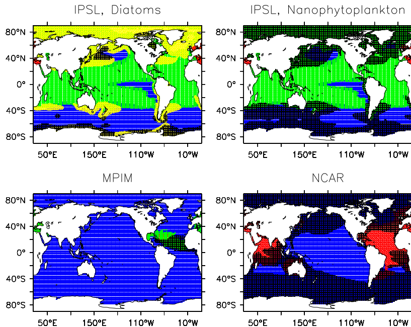
Fig. 5. Maps of variables limiting phytoplankton growth in the models. Blue: iron; red: PO 4 ; green: NO 3 ; yellow: silicate; black: temperature and light. Shown are areas where the respective variable is limiting during at least one month of the year. For nutrients the respective most limiting nutrient is shown, while limitation due to other factors (temperature + light) is shown when nutrients are not limiting, which means the value of the Michaelis-Menten term is above 0.7 (see explanations in the text).
