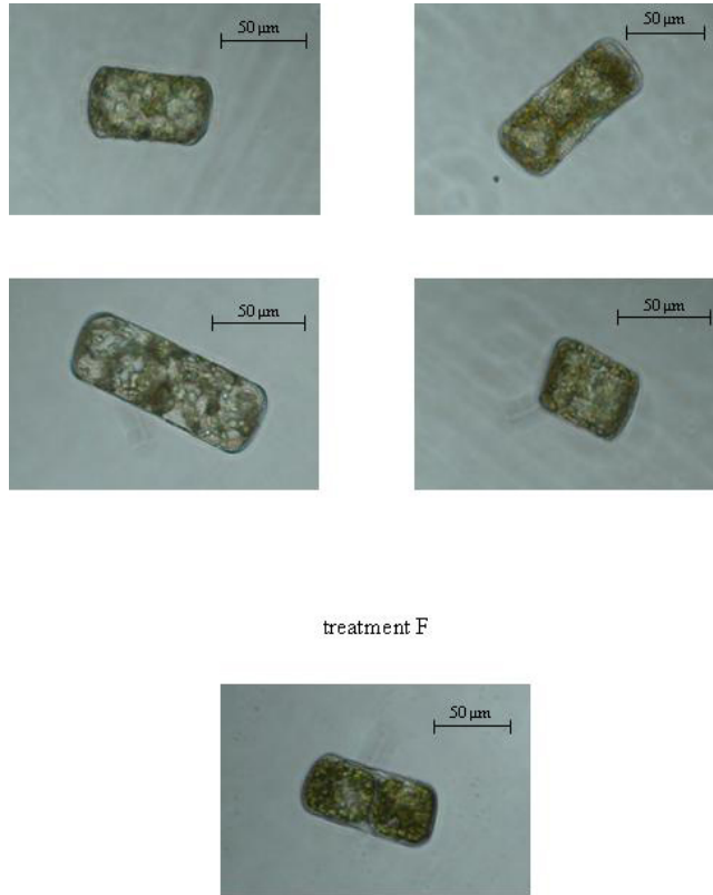
Fig. 3. Light microscopy pictures of Actinocyclus sp. The variance in cell size and Chl content was found in all treatments. In treatment F (picture of dividing cell) all cells had visibly higher Chl concentration per cell.
