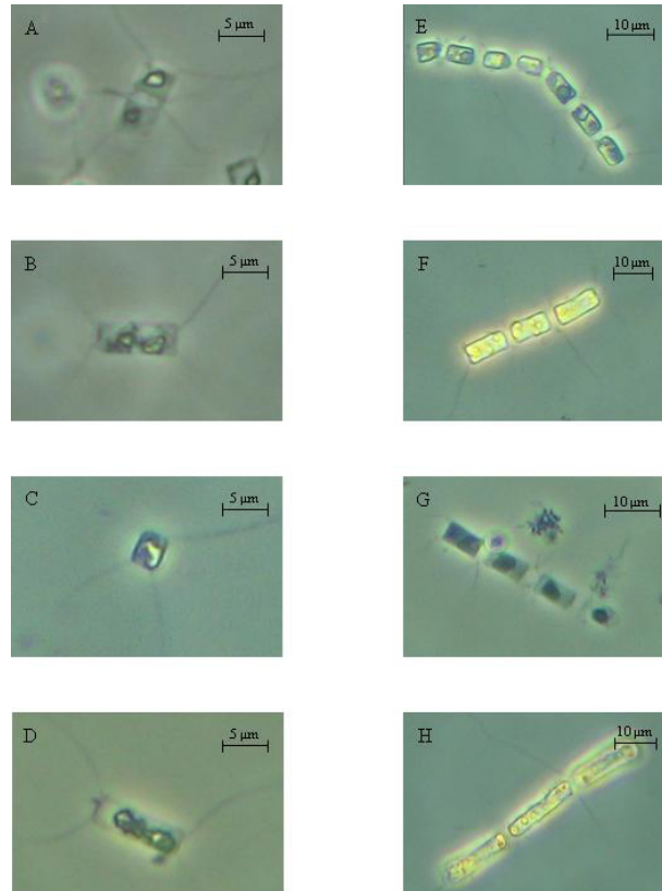
Fig. 1. Light microscopy pictures of C. debilis in the treatments A-H.
