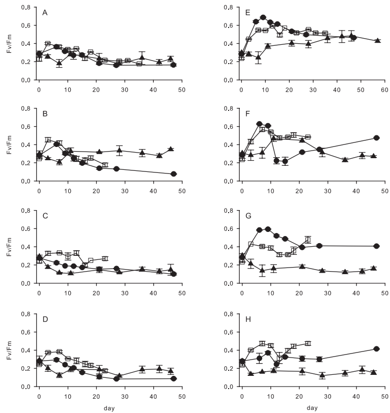
Fig. 5. Fv/Fm of the three species Actinocyclus sp. (dark triangles), Chaetoceros dictaeta (open squares), and C. debilis (dark circles) grown at the eight different treatments A-H. 243
