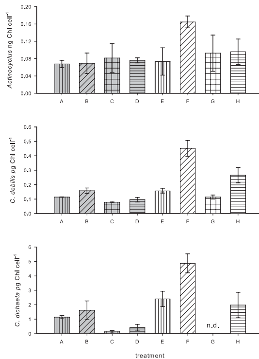
Fig. 6. Cellular chlorophyll concentrations of the three species Actinocyclus sp. (day 46), Chaetoceros dictaeta (day 21), and C. debilis (treatment F and H day 9, all others day 27) grown at the eight different treatments. For the C. dictaeta cultures chlorophyll values for treatment G are missing so no chlorophyll per cell values could be estimated. 244
