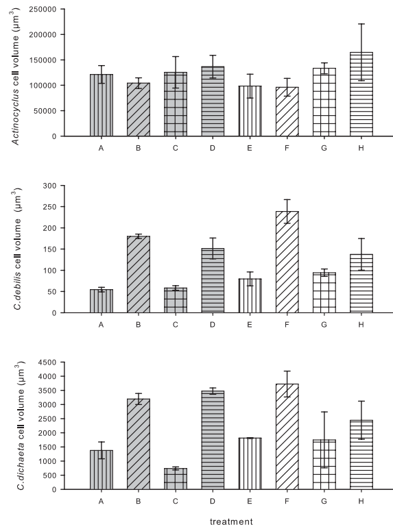
Fig. 7. Cell volume of the three species Actinocyclus sp. (day 46), Chaetoceros dichchaeta (day 21), and C. debilis (day 27) grown at the eight different treatments.
