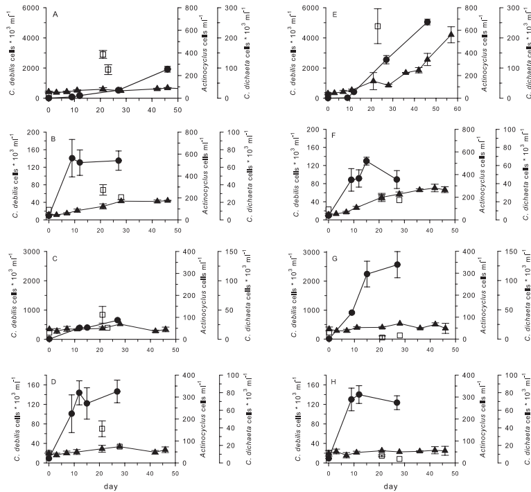
Fig. 4. Cell counts of the three species Actinocyclus sp. (dark triangles), Chaetoceros dichæta (open squares), and C. debilis (dark circles) grown at the eight different treatments A-H. Note different scales for different treatments.
