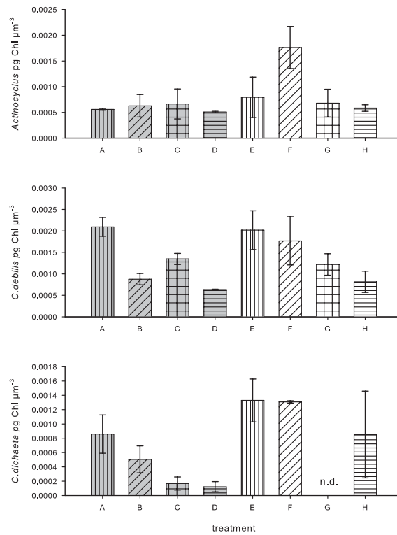
Fig. 8. Chl per cell volume in Actinocyclus (day 46), Chaetoceros dichchaeta (day 21), and C. debilis (day 27) grown at the eight different treatments. For the C. dichchaeta cultures chlorophyll values for treatment G are missing so no chlorophyll per volume values could be estimated.
