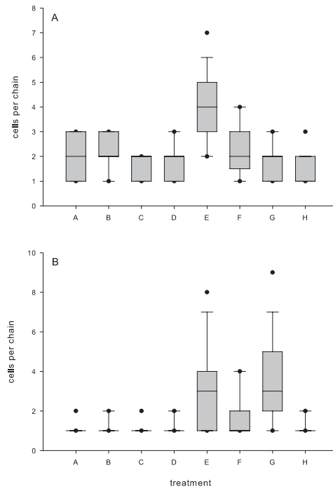
Fig. 9. Chain length of C. dichæta at day 21 (A) and C. debilis (B) at day 9 (treatments A, B), day 12 (treatments F, H and E) and day 15 (treatments C, D, G). The boundary of the box closest to zero indicates the 25th percentile, the line within the box marks the median, and the boundary of the box farthest from zero indicates the 75th percentile. Whiskers (error bars) above and below the box indicate the 90th and 10th percentiles and dark points indicate the 95th and 5th percentile.
