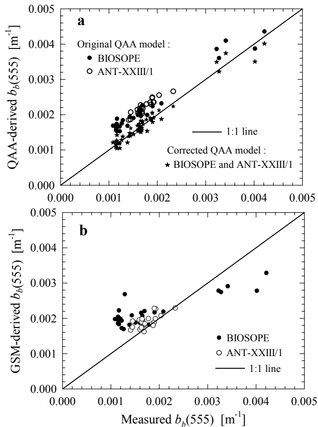
Fig. 9. Particulate backscattering coefficient, b_b(555) , derived from a semianalytical model as a function of measured b_b(555) for (a) a semianalytical model of Lee et al. (2002) referred to as QAA, and (b) a semianalytical model of Garver and Siegel (1997) updated by Maritorena et al. (2002), referred to as GSM. Panel (a) shows the results for both the original QAA model and the corrected QAA model (see text and Table 7 for details). The results in panel (b) are for the GSM model.
