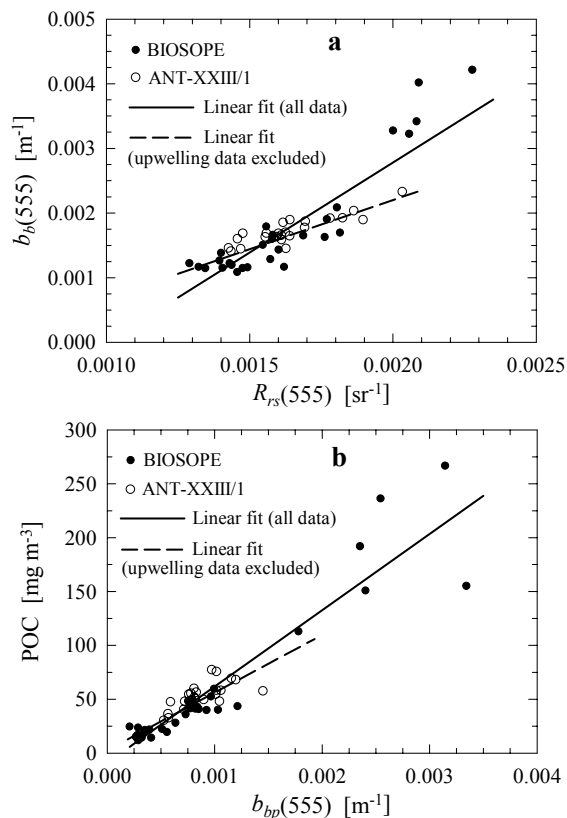
Fig. 7. (a) Relationship between surface values of the backscattering coefficient, b_b(555) , and remote-sensing reflectance, R_{rs}(555) . (b) Relationship between surface concentration of particulate organic carbon, POC, and particulate backscattering coefficient, b_{bp}(555) . The data points for the BIOSOPE and ANT-XXIII/1 cruises and the linear function fits to all data (solid lines) and the limited data sets with Chilean upwelling stations excluded (dashed lines) are shown in both panels (see Table 6 for regression coefficients and error statistics).
