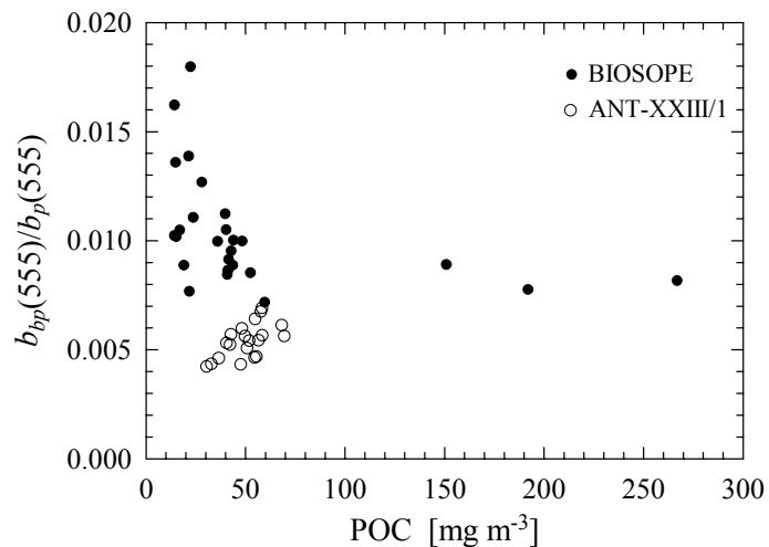
Fig. 10. Particulate backscattering ratio, b_{bp}(555)/b_p(555) , plotted as a function of surface concentration of particulate organic carbon, POC, for the BIOSOPE and ANT-XXIII/1 cruises.
