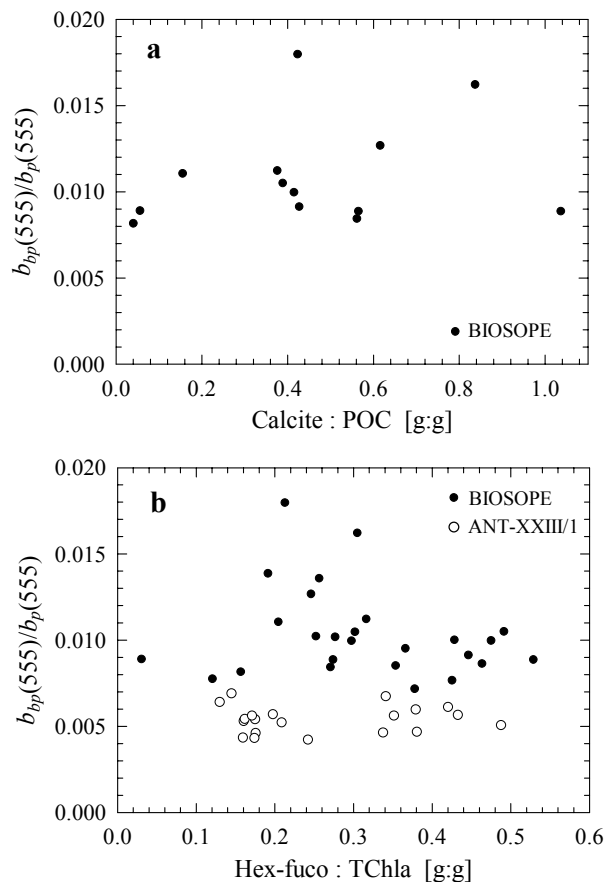
Fig. 11. Particulate backscattering ratio, b_{bp}(555)/b_p(555) , plotted as a function of (a) surface concentration of particulate calcite for the BIOSOPE cruise, and (b) pigment ratio Hex-fuco:TChla in surface waters for the BIOSOPE and ANT-XXIII/1 cruises. The calcite and pigment data for BIOSOPE are taken from Beaufort et al. (2007) and Ras et al. (2007), respectively.
