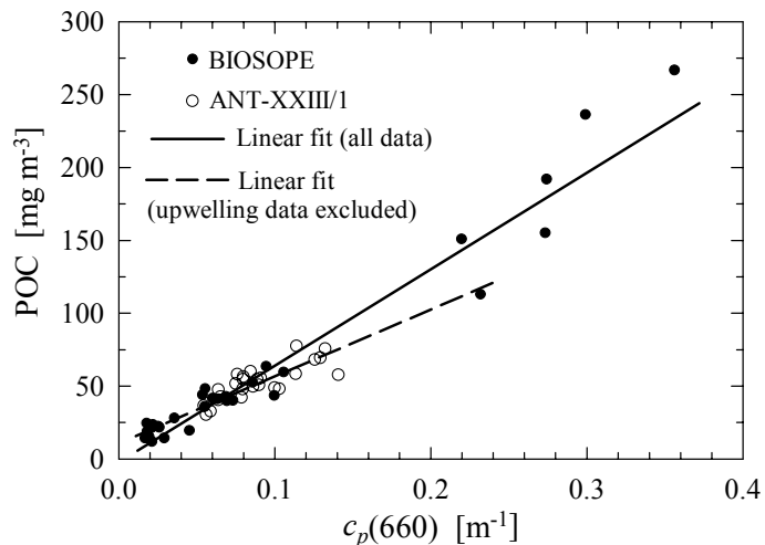
Fig. 6. Relationship between surface concentration of particulate organic carbon, POC, and particulate beam attenuation coefficient, c_p(660) . The data points for the BIOSOPE and ANT-XXIII/1 cruises and the linear function fits to all data (solid line) and the limited data sets with Chilean upwelling stations excluded (dashed line) are shown (see Table 4 for regression coefficients and error statistics).
