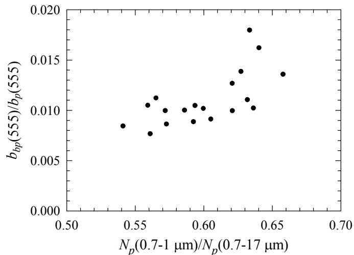
Fig. 12. Particulate backscattering ratio, b_{bp}(555)/b_p(555) , plotted as a function of the contribution of submicrometer particles to the total concentration of particles measured on the BIOSOPE cruise with a Beckman Coulter Multisizer III equipped with a 30\text{-}\mu\text{m} aperture tube. The submicrometer particles are here represented by the concentration of particles, N_p(0.7\text{--}1 \mu\text{m}) , with equivalent diameter between 0.7 and 1 \mu\text{m} , and the total particle concentration, N_p(0.7\text{--}17 \mu\text{m}) , refers to particles in the size range from 0.7 to 17 \mu\text{m} .
