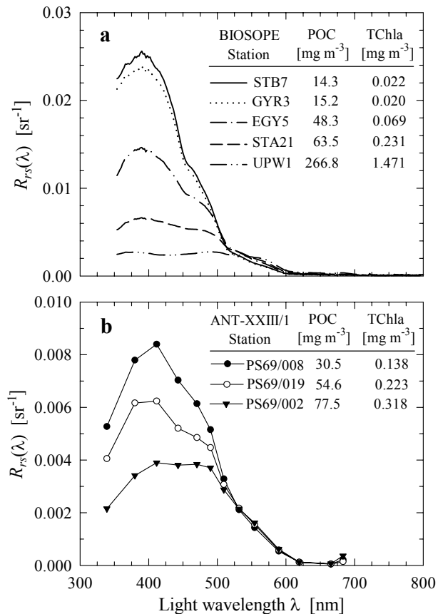
Fig. 3. Example spectra of remote-sensing reflectance, R_{rs}(\lambda) , measured on the BIOSOPE (panel a) and ANT-XXIII/1 (panel b) cruises at stations with different levels of surface particulate organic carbon (POC) and chlorophyll a (TChla) concentrations. The name of the station and the POC and TChla concentrations are indicated.
