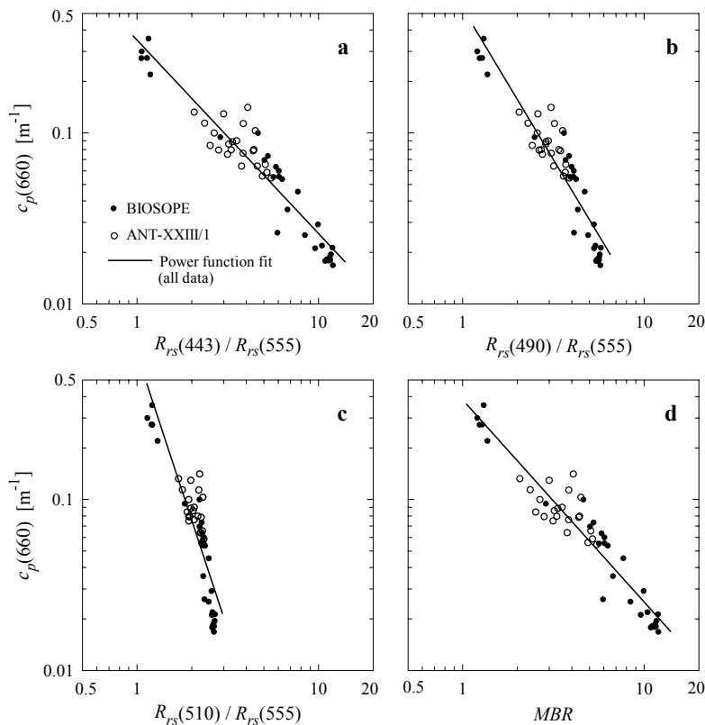
Fig. 5. Relationships between surface values of the particulate beam attenuation coefficient, c_p(660) , and the blue-to-green band ratio of remote-sensing reflectance, R_{rs}(\lambda_B)/R_{rs}(555) . The light wavelength \lambda_B is either 443 nm (panel a ), 490 nm (panel b ), or 510 nm (panel c ), and MBR (panel d ) is the maximum band ratio which refers to the maximum value of the three band ratios considered. The data points for the BIOSOPE and ANT-XXIII/1 cruises and the power function fits to all data are shown in all panels (see Table 4 for regression coefficients and error statistics).
