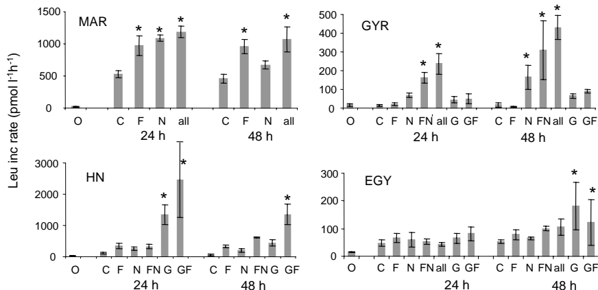
Fig. 2. Evolution of leucine incorporation rates on bioassay experiments made under “trace metal clan” conditions. Means \pm sd of triplicate bottles sampled after 24 and 48 h of incubations. For MAR and HNL enrichments were O: initial conditions, C: control nonenriched, F: +iron, N: + nitrates+ammonium+phosphates+silicates, all: nitrates+phosphates+silicates+iron, G: +glucose, GF: glucose + iron. For GYR and EGYR N was only nitrate+ammonium, FN was nitrate+ammonium+iron and all nitrates+ammonium+phosphates +iron. *: response significantly different from the control at the same time, ANOVA test, p < 0.05 .
