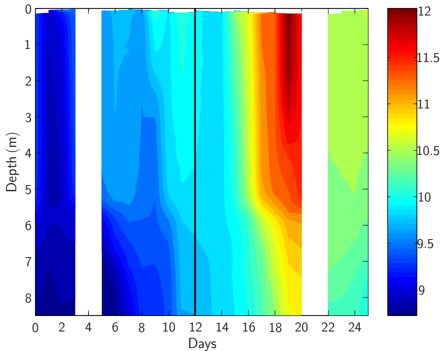
Fig. 3. Temporal changes in the vertical temperature distribution averaged along all nine mesocosms. Standard deviation between mesocosms was generally less than 0.1°C. The vertical black line marks the “storm event” around day 12.
