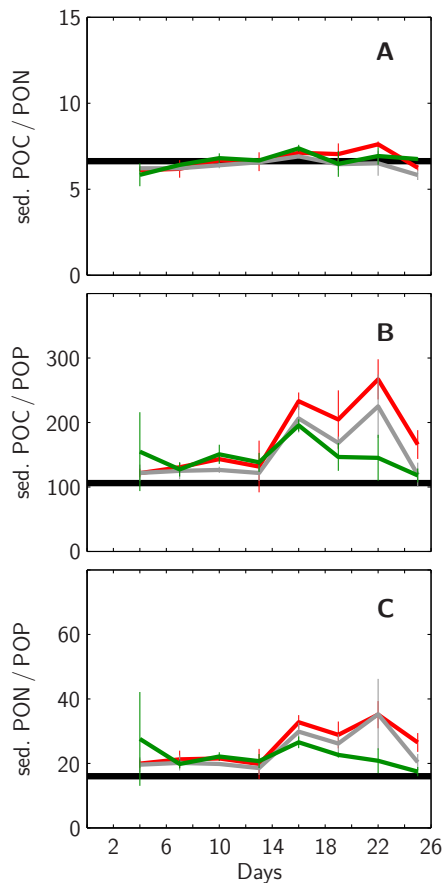
Fig. 11. Temporal development in elemental ratios of particulate organic matter sampled by sediment traps. Shown are sedimentary ratios of POC/PON (A), POC/POP (B), and PON/POP (C). Style and color-coding follow that of Fig. 5. Black horizontal lines denote respective Redfield ratios.
