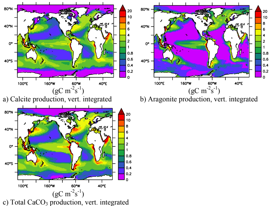
Fig. 2. Production of (a) calcite, (b) aragonite and (c) total \text{CaCO}_3 in \text{gC m}^{-2} \text{s}^{-1} , integrated over depth.
