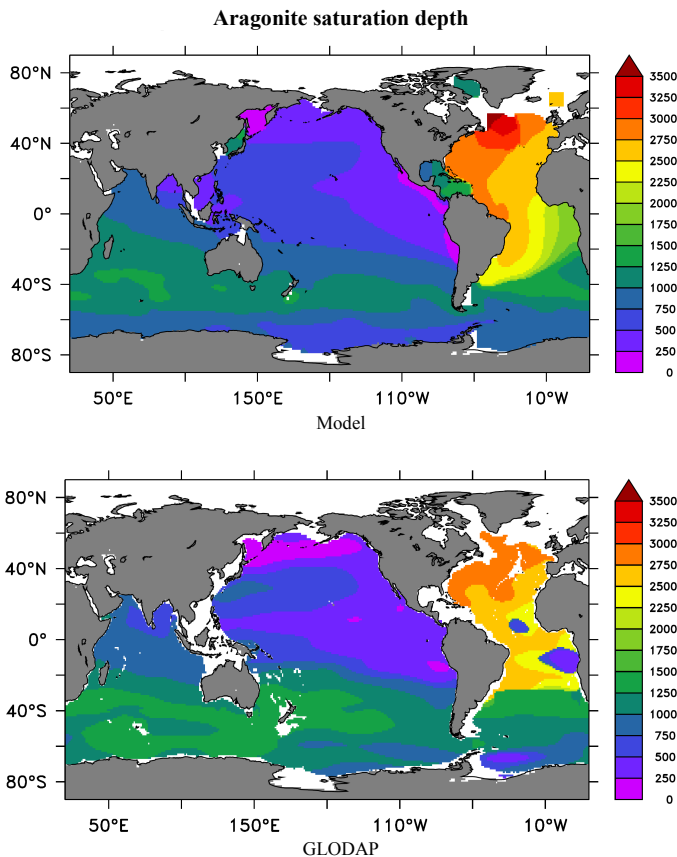
Fig. 1. Depth of aragonite saturation horizon: (a) model output, (b) recalculated from GLODAP (Key et al., 2004).
