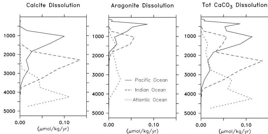
Fig. 3. Average (a) calcite, (b) aragonite and (c) total \text{CaCO}_3 dissolution rates in the Atlantic, Pacific and Indian Ocean basin.
