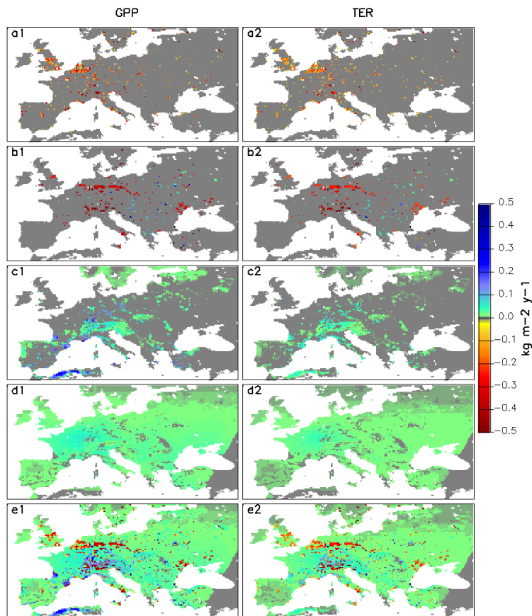
Fig. 5. Response of GPP (a1,b1,c1,d1,e1) and TER (a2,b2,c2,d2,e2) fluxes to different urbanization-driven changes: urban land (a1,a2), urban climate (b1,b2), urban CO 2 dome (c1,c2), elevated nitrogen deposition (d1,d2), and all mentioned changes together (e1,e2).
