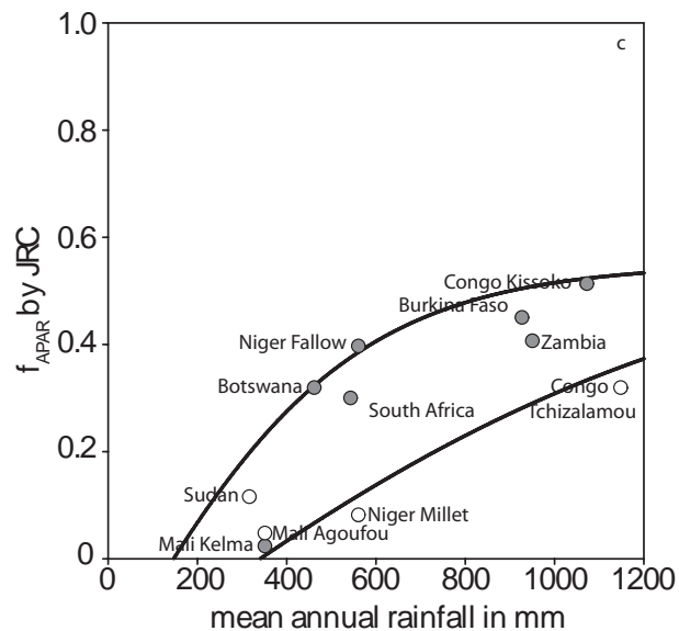
Fig. 8c. The relationship of satellite-derived f_{\text{APAR}} to mean annual rainfall for the analysed sites. The tree dominated ecosystem ( n=6 , grey, Mali-Kelma excluded) lie along the capacity curve, levelling of at 800 mm of rainfall ( y=0.75 \cdot \tanh(x \cdot 0.0014/0.75) - 0.2 ) and the grasslands ( n=4 , white) are explained by the curve below ( y=0.8 \cdot \tanh(x \cdot 0.0006/0.8) - 0.2 ).
