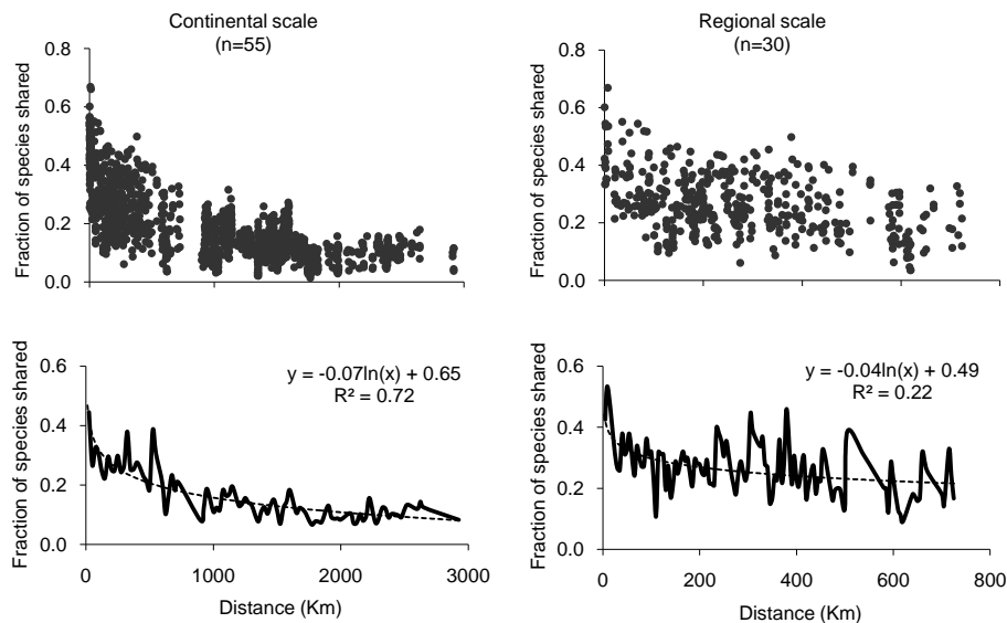
Fig. 3. Floristic similarity (fraction of species shared based on Sørensen’s index) between sample pairs over geographical distance. Top: distribution of values of similarity for each pair of plots. Bottom: averages calculated over 25 km at continental scale and over 5 km at regional scale.
