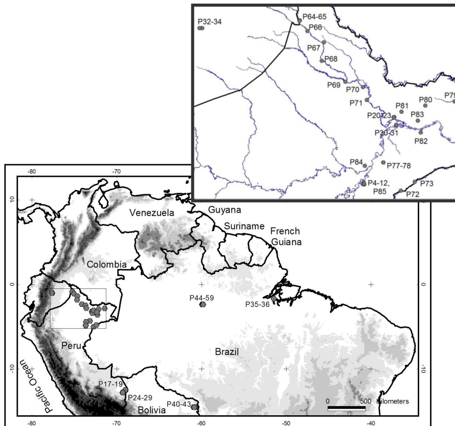
Fig. 1. Location of Amazonian terra firme plots in South America, The Andes are represented in black. Outset shows north-western Amazonian plots. See Table 1 for details of each site.
