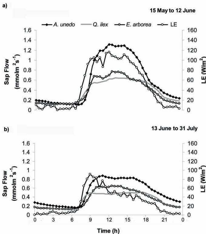
Fig. 3. Average of the half-hourly measurements of sap flow rates of tree species and total ecosystem LE from Eddy Covariance. Values shown are for the mean day of (a) first period and (b) second period. Modified from Gerosa et al. (2009).
