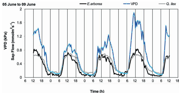
Fig. 5. Daily course of VPD and sap flow of Q. ilex , and E. arborea from 5 to 9 June 2007.
