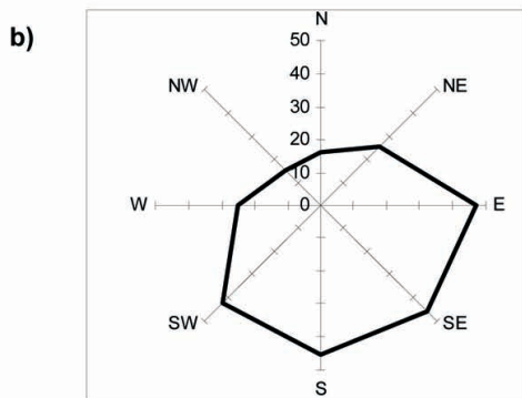
Fig. 2. (a) Average of the half-hourly measurements of ozone concentrations at 1.5 m height. (b) Night-time ozone concentration as function of wind direction. Concentrations are higher when the wind is blowing from the sea.
