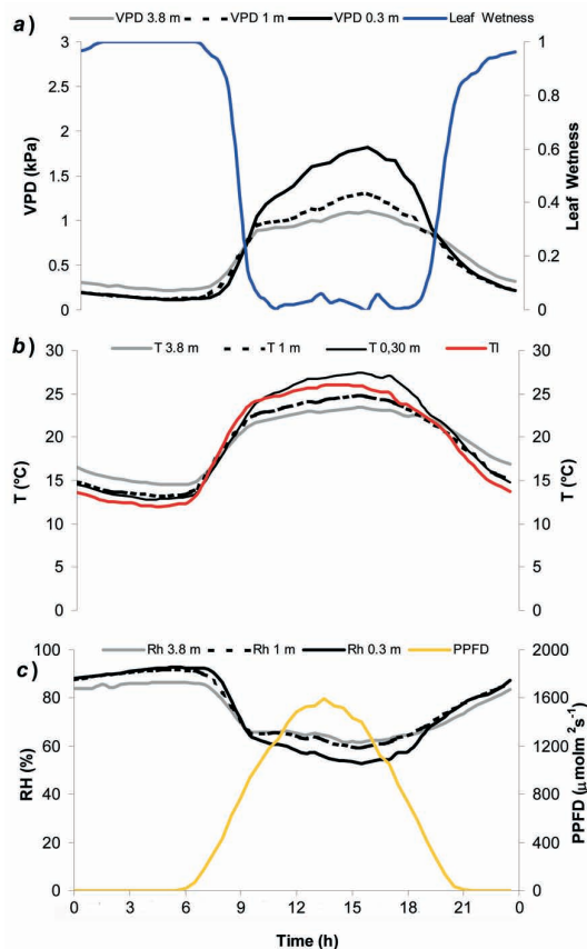
Fig. 1. Average of the half-hourly measurements of environmental parameters calculated using data from the entire experimental campaign (from 15 May to 31 July 2007). (a) Vapour Pressure Difference (VPD, kPa) at tree different heights (3.8 m; 1 m; 0.3 m), and Leaf Wetness (relative frequencies). (b) Air temperature T_a , (°C – 3.8 m; 1 m; 0.3 m) and leaf temperature T_l (°C). (c) Relative Humidity (RH, % – 3.8 m; 1 m; 0.3 m) and solar radiation (PPFD, \mu\text{g mol m}^{-2} \text{s}^{-1} ).
