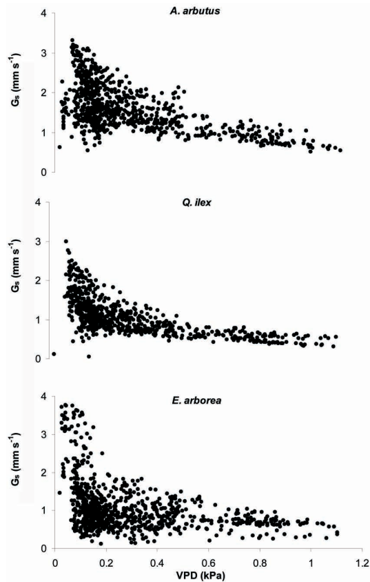
Fig. 7. Relationship between canopy stomatal conductance ( G_s ) and vapour pressure deficit (VPD) for each species using data collected at night (11:00 p.m. to 6:00 a.m.).
