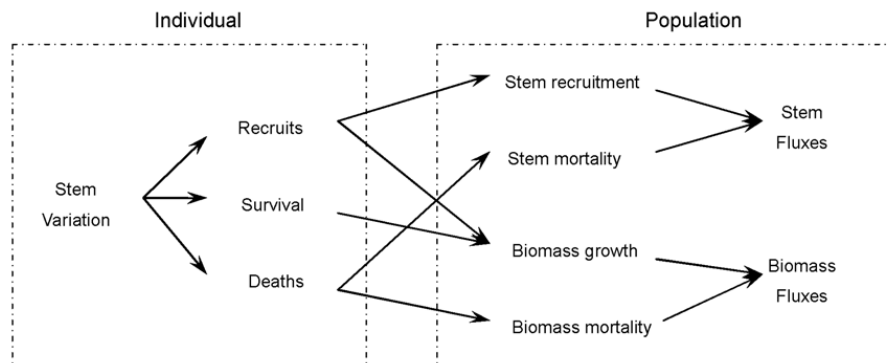
Fig. 1. Diagram for calculating stem and biomass fluxes.
