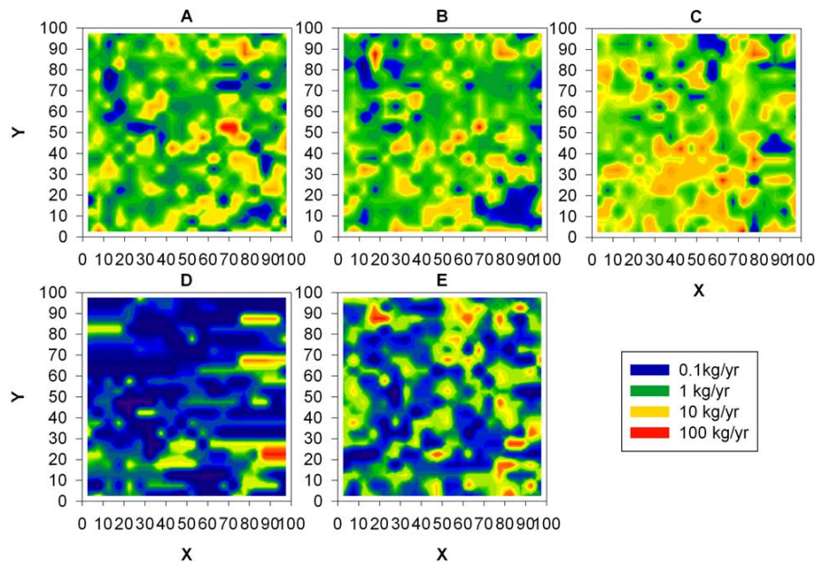
Fig. 9. Filled contour maps for biomass fluxes ( \text{kg} \times \text{yr}^{-1} ) of each subplot as indicated by (A) biomass growth in interval I, (B) biomass growth in interval II, (C) biomass growth in interval III, (D) biomass mortality in interval II and (E) biomass mortality in interval III.
