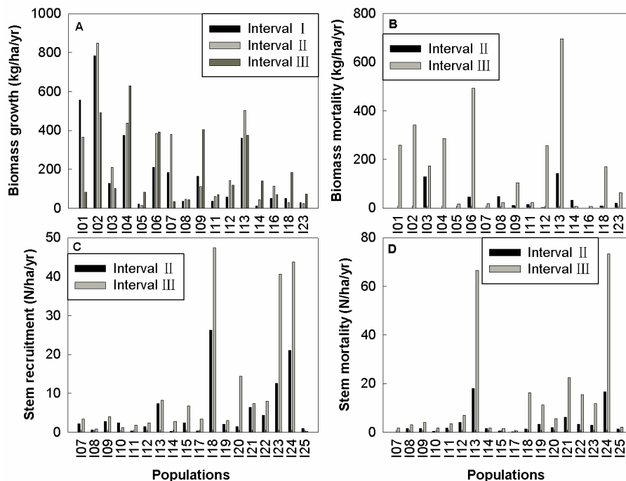
Fig. 6. Biomass and stem fluxes of each dominant population as indicated by (A) biomass growth, (B) biomass mortality, (C) stem recruitment and (D) stem mortality.
