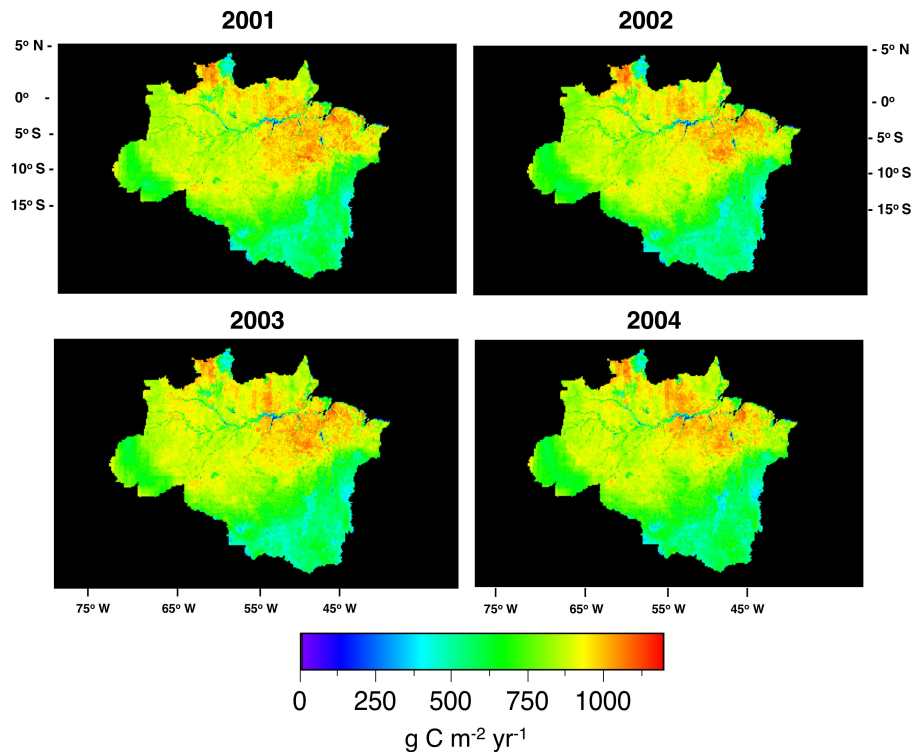
Fig. 2. Predicted annual NPP fluxes from the CASA model for the Legal Amazon over the years 2001–2004.
