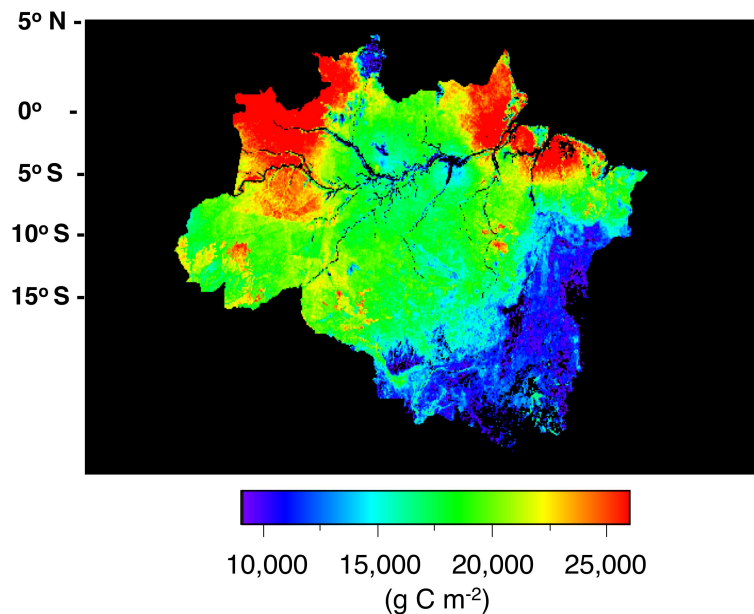
Fig. 3. Predicted aboveground wood biomass pools of carbon from the CASA model for the Legal Amazon, circa 2000.
