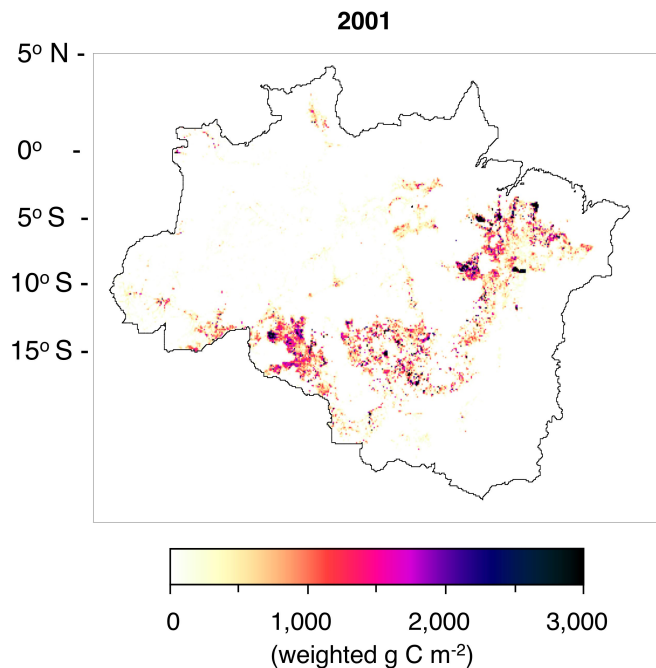
Fig. 6. Biomass burning fluxes of carbon for the Legal Amazon in 2001, based on PRODES deforestation mapping (Fig. 4) and CASA model aboveground wood biomass pools of carbon (Fig. 3).
