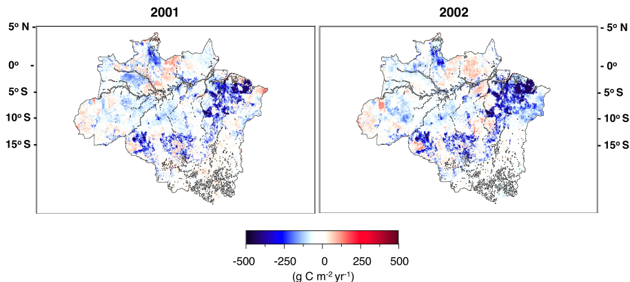
Fig. 7. Predicted annual NEP fluxes from the NASA-CASA model plus emission sources of CO 2 from down wood pools following deforestation in 2001 and 2002 over the Brazilian Amazon region, for estimates of annual NBP fluxes of carbon.
