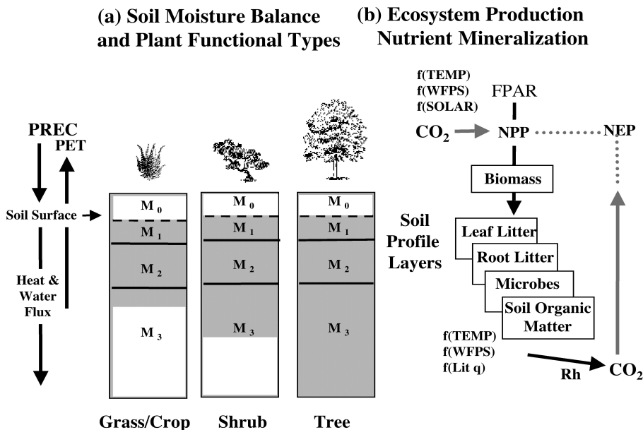
Fig. 1. Schematic representation of components in the NASA-CASA model. The soil profile component [I] is layered with depth into a surface ponded layer (M 0 ), a surface organic layer (M 1 ), a surface organic-mineral layer (M 2 ), and a subsurface mineral layer (M 3 ), showing typical levels of soil water content (shaded) in three general vegetation types (DeFries et al., 1995). The production and decomposition component [II] shows separate pools for carbon cycling among pools of leaf litter, root litter, woody detritus, microbes, and soil organic matter, with dependence on litter quality ( q ).
