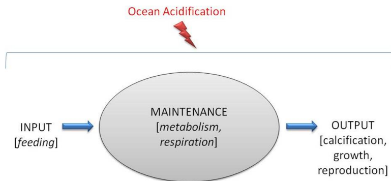
Fig. 2. OA can directly or indirectly affect many physiological processes with consequences on fitness.
