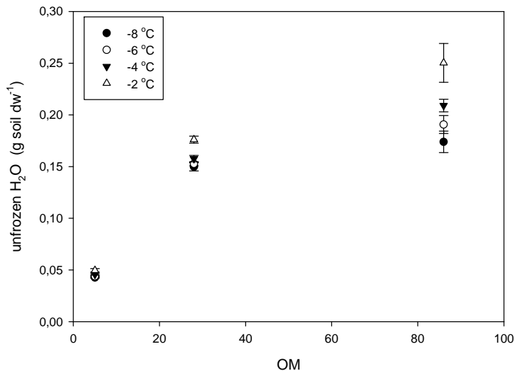
Fig. 6. Amount of unfrozen H 2 O (g soil dw -1 ) plotted against soil organic matter (OM) at different temperatures with standard deviation ( n=6 ).
