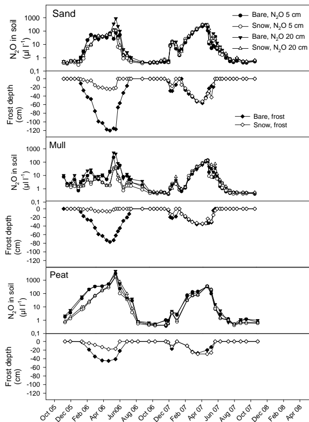
Fig. 2. N 2 O concentration in soil at the depth of 5 cm (circles) and 20 cm (triangles) and the depth of soil frost (diamonds) in sand, mull and peat soils. Black symbols refer bare soil without snow and open symbols soil with undisturbed snow cover during the winter. Error bars show the standard error of the mean. Note the log scale in y-axis (N 2 O in soil).
