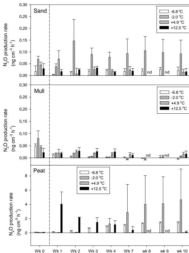
Fig. 5. N 2 O production rates in laboratory incubations with sand, mull and peat soil ( n =5) at temperatures of −6.8, −2.0, 4.9 and 12.5°C. Wk 0 refers the beginning of the incubations at +4.9°C at soil WFPS 80%. Error bars show the standard deviation of the mean. (nd=not determined).
