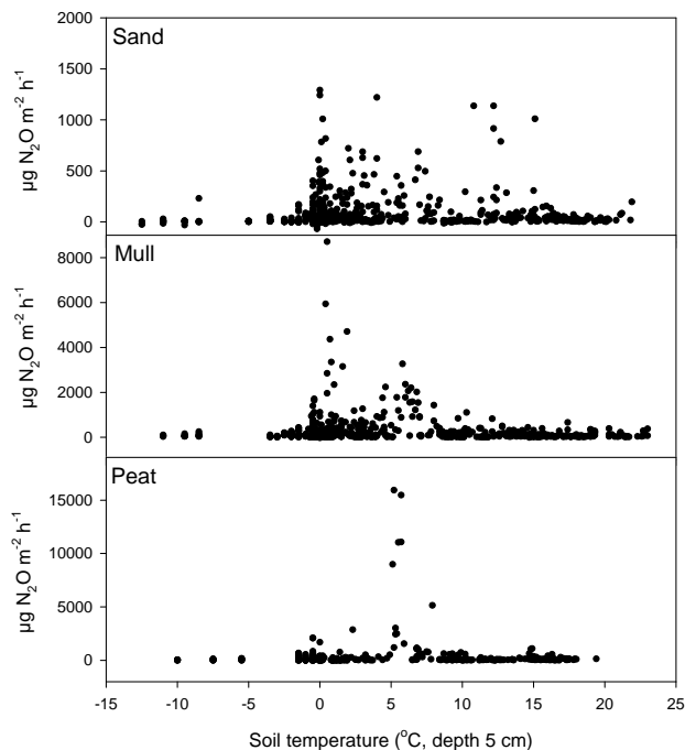
Fig. 3. N 2 O emissions from all individual measurements from sand, mull and peat soils plotted against soil temperature at depth of 5 cm.
