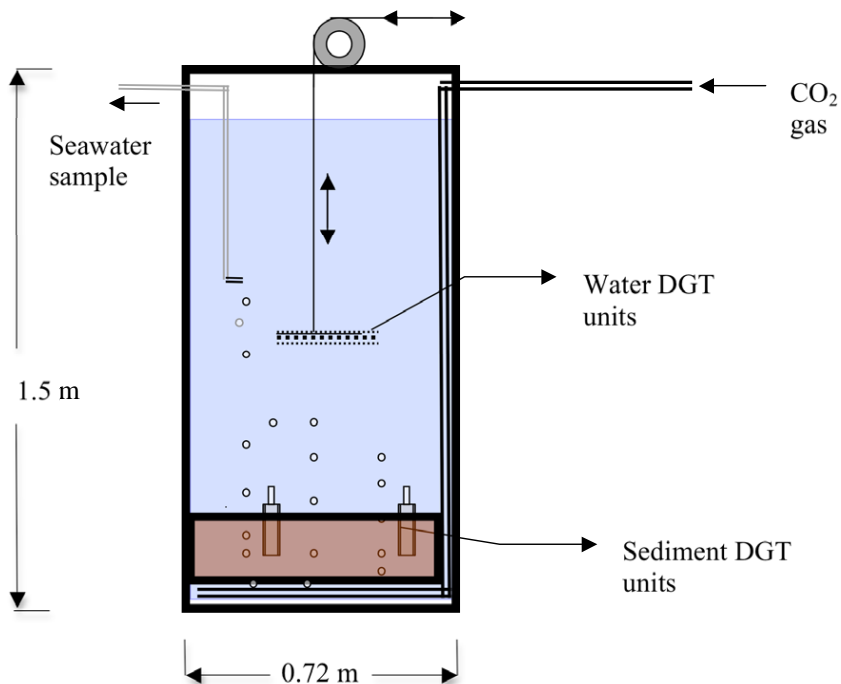
Fig. 1. Schematic representation of the CO 2 seepage chamber.
