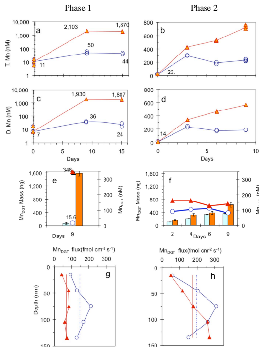
Fig. 4. Concentrations of total acid-leachable Mn (TMn), dissolved Mn (DMn) and DGT labile Mn ( Mn_{DGT} ) in water during the first (a, c, and e) and second (b, d and f) phases in CO 2 seepage (full triangles) and in the control (open circles) chambers. Note that scales of TMn and DMn in the first phase of the experiment (a and c) are logarithmic. The amounts of Mn collected in the DGT units are shown by columns (e and f): light columns for control, dark columns for CO 2 chambers. Flux of Mn_{DGT} from the sediment and pore water into DGT units in different sections of the sediment during the first (g) and second (h) phases of the experiment are shown as full triangles and open circles for CO 2 seepage control chamber, respectively. The total average flux of Mn_{DGT} in the sediment for CO 2 and control chambers is indicated by a broken line and dotted line, respectively.
