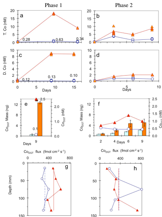
Fig. 5. Concentrations of total acid-leachable Co (TCo), dissolved Co (DCo) and DGT labile Co ( Co_{DGT} ) in water during the first ( a , c , and e ) and second ( b , d and f ) phases of the experiment in CO 2 seepage (full triangles) and in the control (open circles) chambers. The amounts of Co collected in the DGT units are shown by columns ( e and f ): light columns for control, dark columns for CO 2 chambers. Flux of Co_{DGT} from the sediment and pore water into DGT units in different sections of the sediment during the first ( g ) and second ( h ) phases of the experiment are shown as full triangles and open circles for CO 2 seepage control chamber, respectively. The total average flux of Co_{DGT} in the sediment for CO 2 and control chambers is indicated by a broken line and dotted line, respectively.
