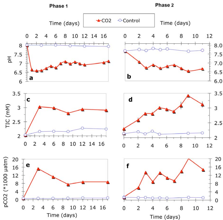
Fig. 2. Variation of pH (a and b), total inorganic carbon, TIC (c and d), and partial pressure/fugacity of CO 2 ( p\text{CO}_2 ) (e and f) during both phases of the experiment in CO 2 seepage (full triangles) and in the control (open circles) chambers.
