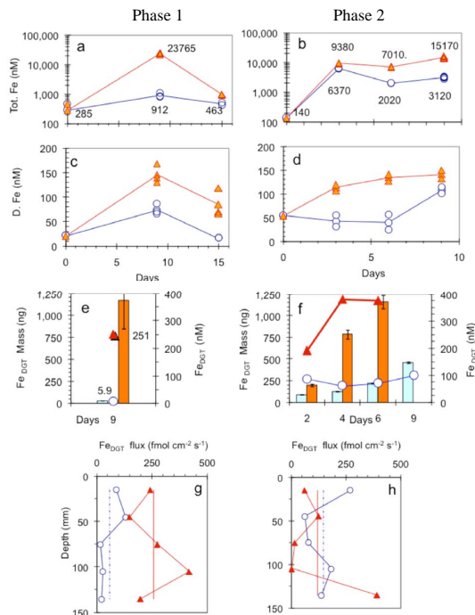
Fig. 3. Concentrations of total acid-leachable Fe (TFe), dissolved Fe (DFe) and DGT labile Fe ( \text{Fe}_{\text{DGT}} ) in water during the first (a, c, and e) and second (b, d and f) phases of the experiment in CO 2 seepage (full triangles) and in the control (open circles) chambers. Note that scales of TFe are logarithmic (a, b). The amounts of Fe collected in the DGT units are shown by columns (e and f): light columns for control, dark columns for CO 2 chamber. Flux of \text{Fe}_{\text{DGT}} from the sediment and pore water into DGT units in different sections of the sediment during the first (g) and second (h) phases of the experiment are shown as full triangles and open circles for CO 2 seepage control chamber, respectively. The total average flux of \text{Fe}_{\text{DGT}} into hole DGT unit in the sediment for CO 2 and control chambers is indicated by a broken line and dotted line, respectively.
