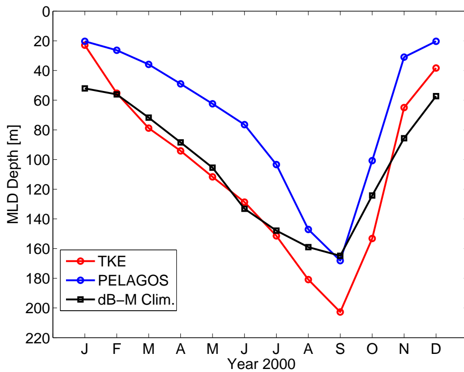
Fig. 1. Results of the sensitivity experiment on the artificial increase of TKE in the Southern Ocean (year 2000). Comparison of the seasonal cycle of mixed layer depths in the Subantarctic province
