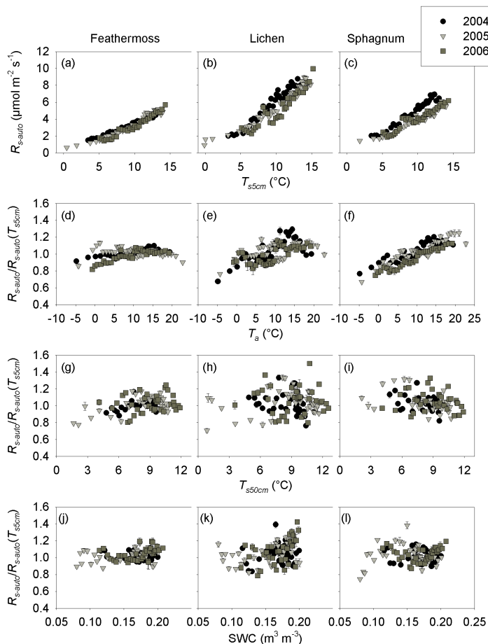
Fig. 3. Relationships between soil temperature at 5 cm depth ( T_{s5cm} ) and automated soil respiration ( R_{s-auto} ) under (a) feathermoss, (b) lichen and (c) sphagnum ground cover. Relationships of R_{s-auto} normalized for T_{s5cm} ( R_{s-auto}/R_{s-auto}(T_{s5cm}) ) with (d–f) air temperature ( T_a ), (g–i), soil temperature at 50 cm depth ( T_{s50cm} ) and (j–l) soil water content (SWC) for the three forest floor cover types. Binned data \pm SE ( n=100 ) are presented.
