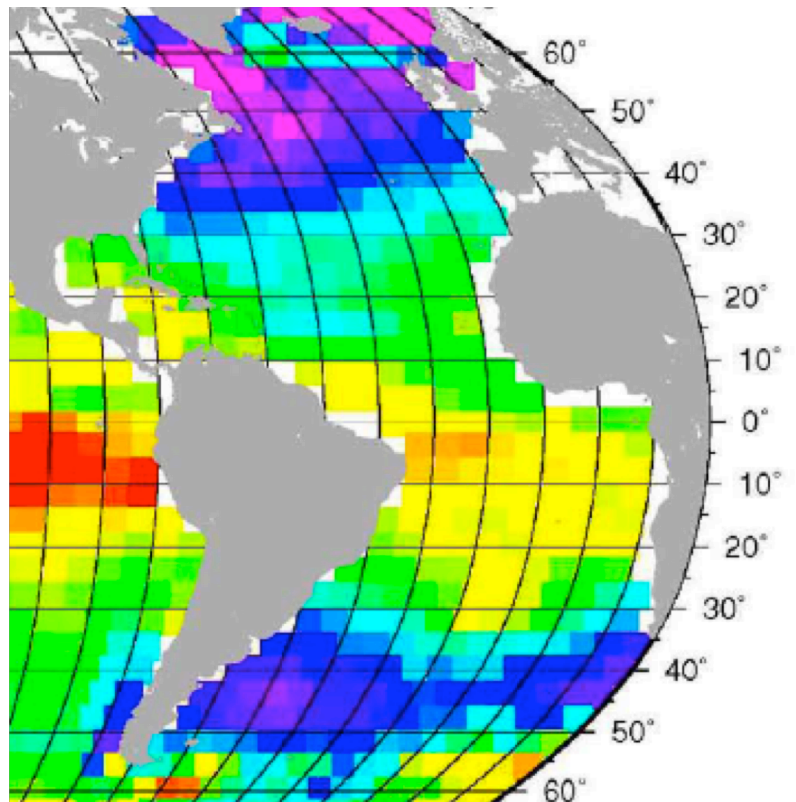
Net flux of CO 2 in the Atlantic Ocean (Takahashi et al., 2009)
