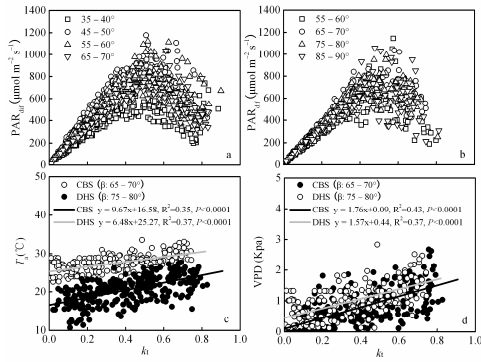
Fig. 6. Changes of diffuse PAR (PAR diff ) at (a) CBS, (b) DHS, (c) air temperature (T a ) and (d) vapor pressure deficit (VPD) with the clearness index (k t ) for selected intervals of solar elevation angles from June to August in 2005.
