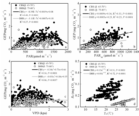
Fig. 7. Changes of GEP with (a) PAR, (b) diffuse PAR (PAR diff ), (c) VPD and Changes of (d) R e with air temperature (T a ) for selected intervals of solar elevation angles at CBS and DHS from June to August in 2005.
