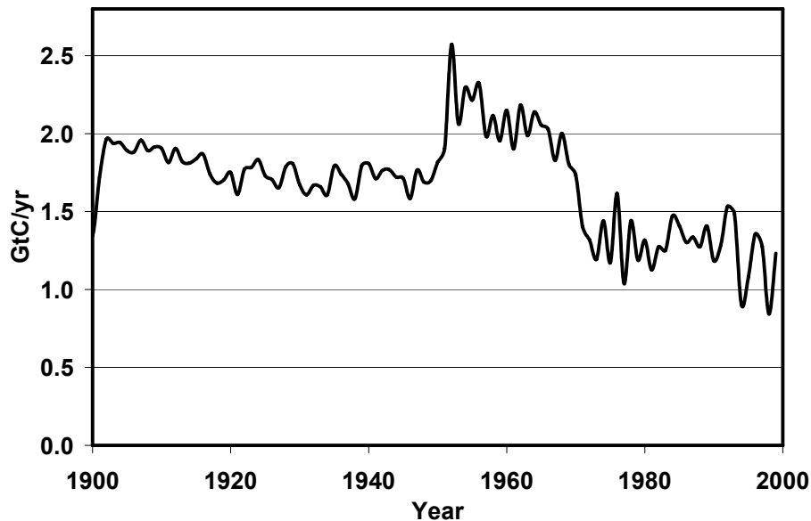
Fig. 1. ISAM estimated annual global mean emissions from land use change (GtC/year) for the period 1900–2000.
