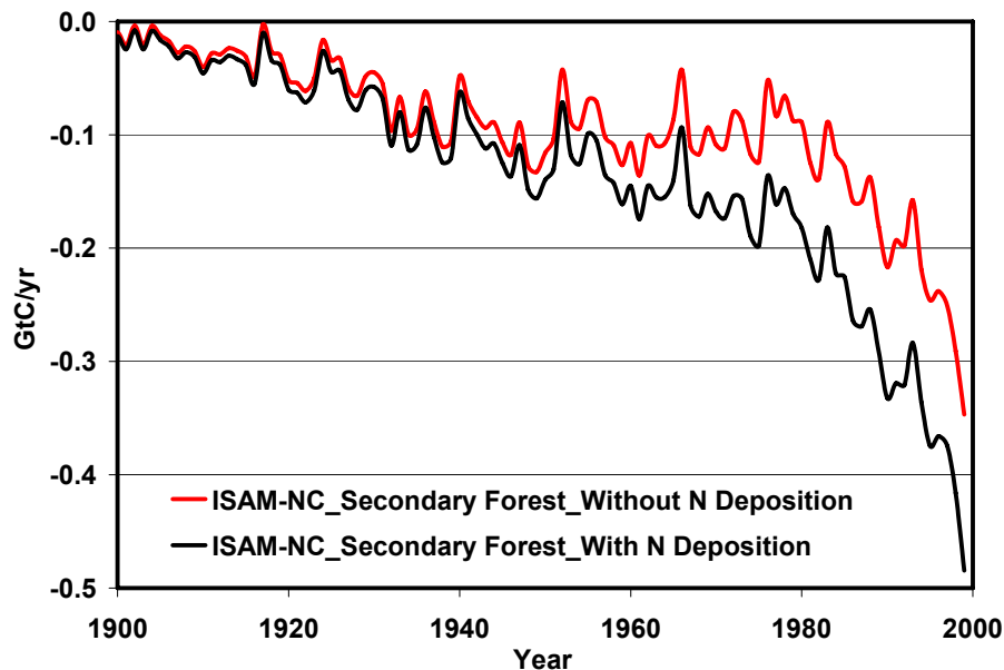
Fig. 4. Global net carbon flux (GtC/a) in secondary forests comparing ISAM-NC including N deposition and ISAM-NC-without N deposition between 1900 and 2000. Positive values represent net C release to the atmosphere and negative values represent net C storage in terrestrial biosphere.
