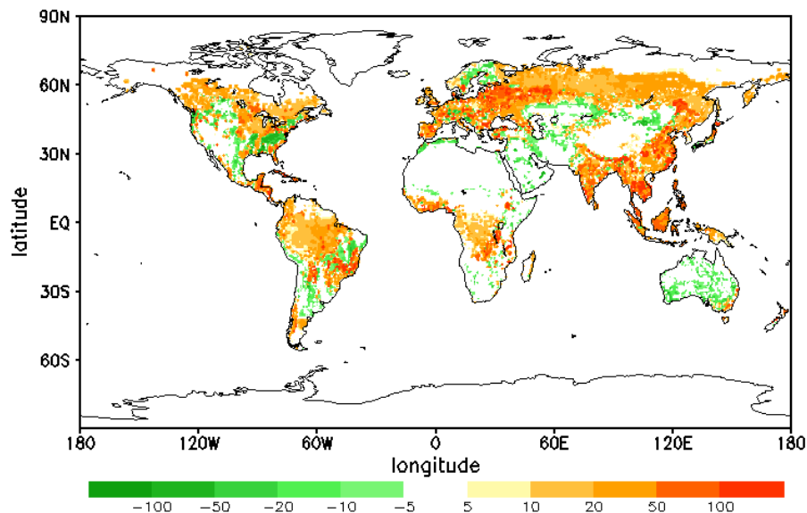
Fig. 2. ISAM estimated spatial distributions of carbon emissions from land use change in the 1990s (Unit: \text{gC}/\text{m}^2/\text{yr} ). Positive values represent net C release to the atmosphere and negative values represent net C storage in the terrestrial biosphere.
