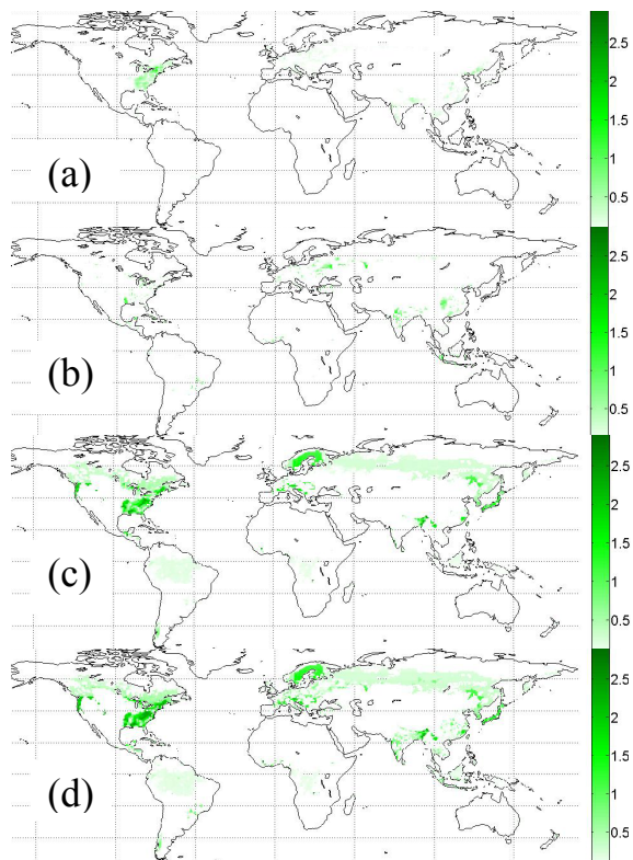
Fig. 3. The distribution of secondary forest area ( 10^9 \text{ m}^2 ) regrown from (a) cropland abandonment, (b) pastureland abandonment, (c) wood harvest, and (d) sum of (a), (b) and (c).
