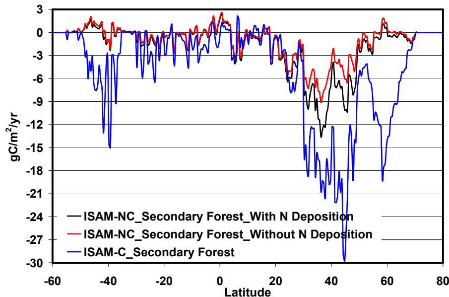
Fig. 5. Latitudinal distribution of net carbon flux ( \text{gC/m}^2/\text{yr} ) for the 1990s in secondary forests for ISAM-NC with N deposition, ISAM-NC without N deposition and ISAM-C. In ISAM-NC experiments, C fluxes are affected by N dynamics, whereas in ISAM-C experiment C fluxes are not affected by N dynamics. Positive values represent net C release to the atmosphere and negative values represent net C storage in terrestrial biosphere.
