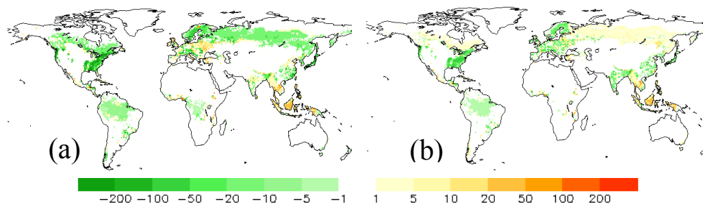
Fig. 6. Spatial distributions of the net exchange of carbon ( \text{gC}/\text{m}^2/\text{yr} ) for the 1990s in secondary forests for (a) ISAM-C and (b) ISAM-NC. C fluxes estimated based on ISAM-C version of the model are not constrained by N dynamics, whereas ISAM-NC based C fluxes are constrained by the N dynamics. Positive values represent net C release to the atmosphere and negative values represent net C storage in terrestrial biosphere.
