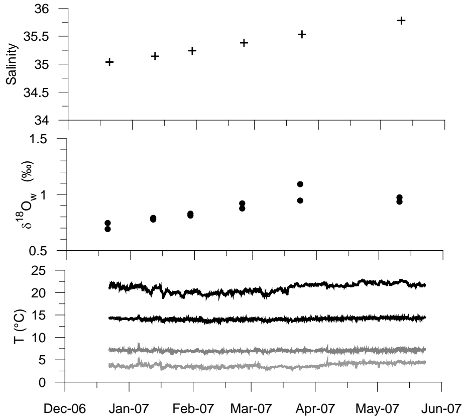
Fig. 2. Salinity, \delta^{18}O_w , and temperature measured during the experiment. Two water samples from the reservoir tank were taken for salinity and \delta^{18}O_w at each sampling occasion, temperature was measured continuously with data loggers.
