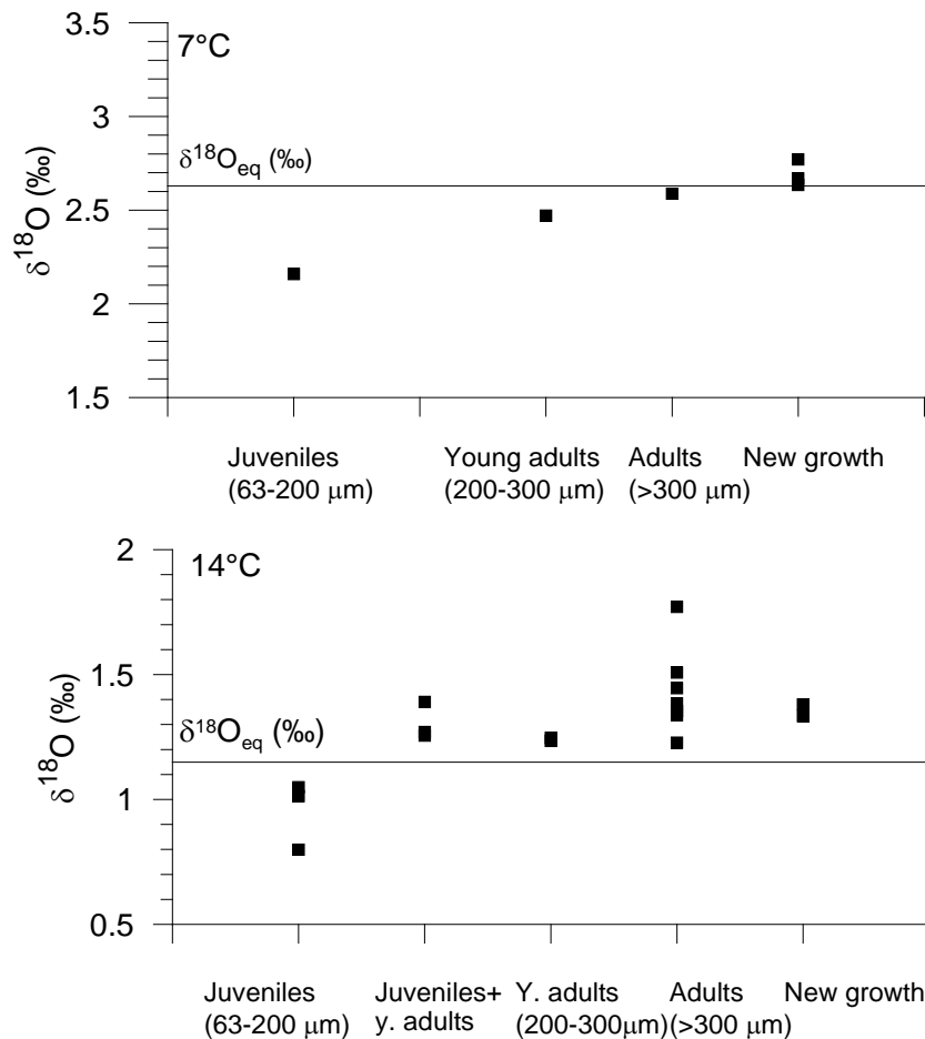
Fig. 4. The uppermost panel (A) shows \delta^{18}\text{O} values at 7°C and the lower panel (B) for 14°C for the different size classes, together with the equilibrium calcite line for each temperature.
