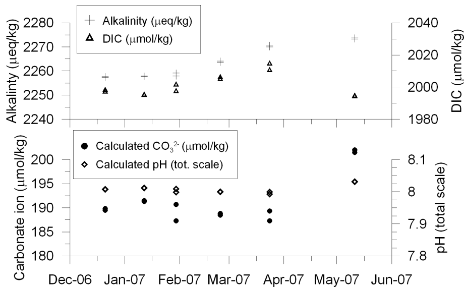
Fig. 3. Water chemistry data during the course of the experiment. Alkalinity and DIC were analyzed from water samples from the reservoir tank, and used to calculate [CO 3 2- ] and pH(t).
