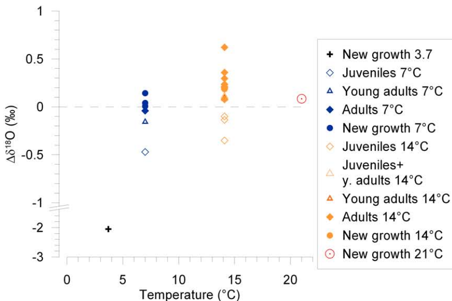
Fig. 6. The difference between \delta^{18}\text{O}_c and the \delta^{18}\text{O}_{(eq)} vs. experimental temperature. \delta^{18}\text{O}_{(eq)} is indicated with a dotted line and calculated using the Bemis et al. (1998) paleotemperature equation, together with a \delta^{18}\text{O}_w of 0.92‰ (average between February and May). All calcite was precipitated during the experiment; the symbols refer to the different material, see legend for details.
