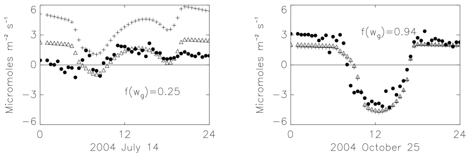
Fig. 3. Comparison of NEE simulations of ISBA-A-gs based on R_{eco} calculated from either Eq. (1) or Eq. (4) (+ and triangles, respectively), with NEE observations (dots), for two days presenting contrasting soil moisture conditions: (left) 14 July 2004, (right) 25 October 2004.
