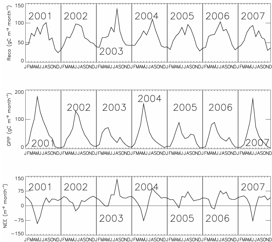
Fig. 6. A seven-year (2001–2007) simulation by ISBA-A-gs of monthly values of (from top to bottom): R_{\text{eco}} , GPP, and NEE.
