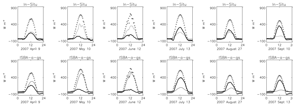
Fig. 5. Observed (top) and simulated (bottom) energy fluxes for 6 daily cycles in April, May, June, July, August, September 2007: Rn (dots), H (thick), LE (fine line).
