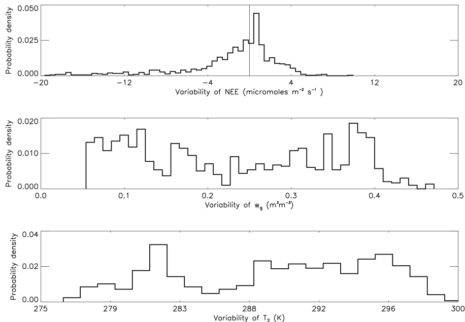
Fig. 1. Variability of the net CO 2 flux, w_g and T_2 for wind direction between 225 and 315 degrees, sufficient turbulent exchange ( u^* > 0.16 \text{ ms}^{-1} ), and in the absence of water deposition, for pooled daytime and nighttime data.
