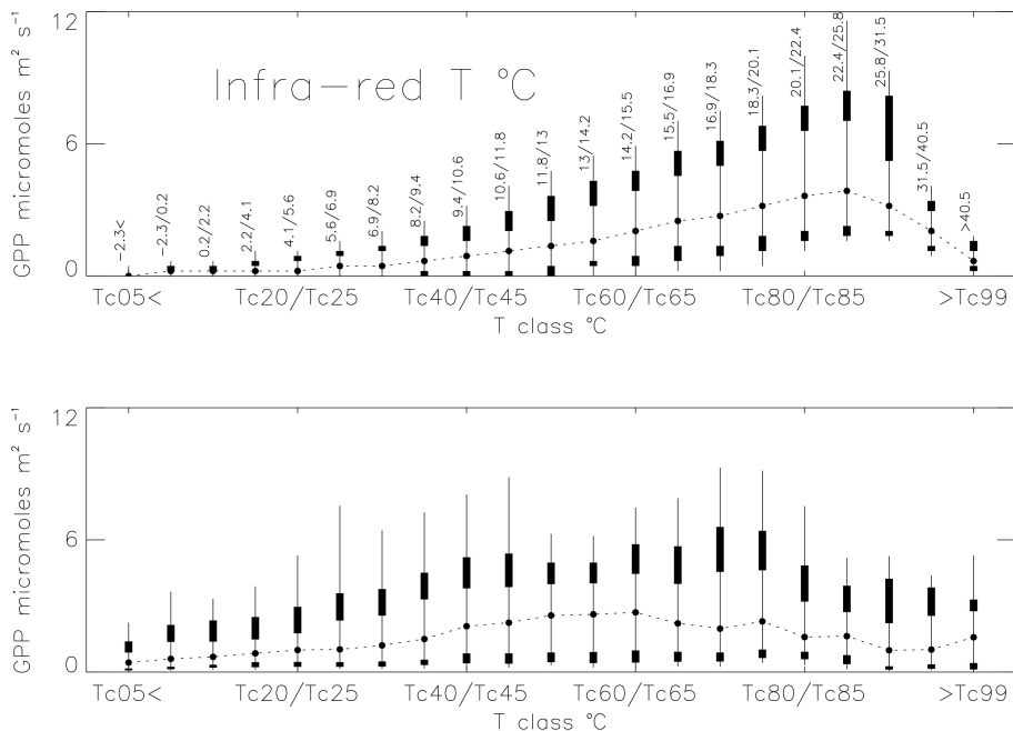
Fig. 4. Response of (top) the simulated GPP and of (bottom) the estimated GPP, to the observed surface infrared-derived temperature. The median difference (dots) is presented together with percentile values. Line: 5–95% percentile, closed box (bottom) 10–20% percentile, closed box (top) 80–90% percentile. GPP statistics are given for 21 temperature classes ( T_c ) corresponding to 5% percentile intervals.
