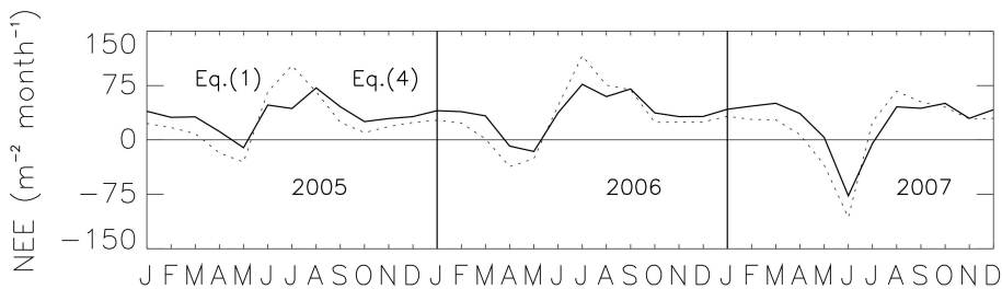
Fig. 2. Monthly NEE (sum of the net CO 2 flux) simulated by ISBA-A-gs using R eco calculated from either Eq. (1) or Eq. (4) (dashed and solid line, respectively).
