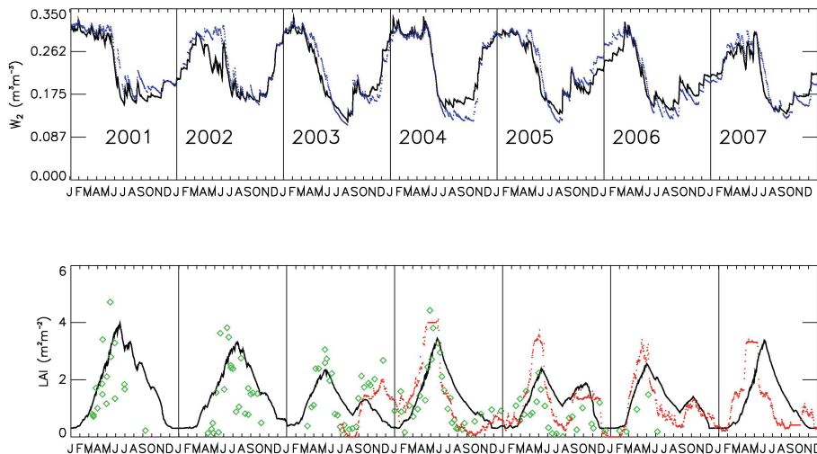
Fig. 7. Root-zone soil moisture ( w_2 ), and leaf area index (LAI) of the SMOSREX grassland for a seven year (2001–2007) period, simulated by ISBA-A-gs (black solid lines) and observed (blue dots for soil moisture, green diamonds for LAI estimates derived from destructive measurements, red dots for LAI estimates derived from surface reflectance measurements).
