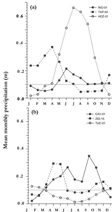
Fig. 3. Precipitation patterns for selected sites showing different patterns associated with dry season length, S_D and precipitation coefficient of variation, P_V . (a) variations in, P_V possible with S_D=4 months. RIO-01; Rio Grande, Venezuela (Guyanan Shield), P_V = 0.41 , mean annual precipitation, P_A = 1.35 m; TAP-04; Tapajos, Brazil (Central/Eastern Brazil), P_V = 0.65 , P_A = 2.02 m, HOZ-01; Chékô, Cambodia, Hozumi (Asia), P_V = 0.86 , P_A = 3.34 m. (b) : observed variations in, S_D , but with all sites all having P_V=0.56 . CAV-01; Cavalla, Liberia (West Africa) S_D = 3 months, P_A = 1.96 m; ZIG-15; Zigi Forest, Tanzania (East Africa), S_D = 6 months, P_V = 1.62 m; TUC-01; Tucavaca, Bolivia (Southern Amazon), S_D = 9 months, P_A = 0.82 m.
