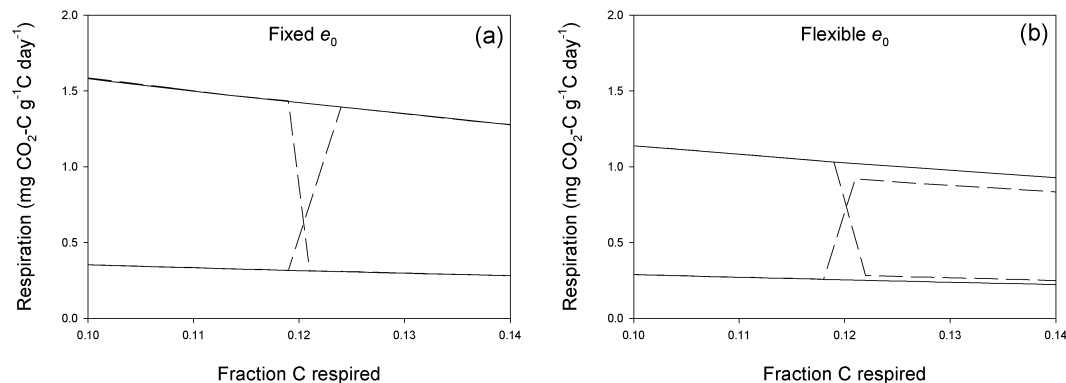
Fig. 3. Respiration rates of samples as a function of fraction of respired carbon, predicted by the flexible and fixed decomposer efficiency models with constant temperatures (solid lines) and with a switch between 5 and 25 °C at 12% respired carbon (broken lines) using the parameter set with the highest LM (Table 1). For clarity, the transitions between temperatures are slightly displaced from exactly 12%. (a) Fixed e_0 . (b) Flexible e_0 . Note, these simulations do not give the same result as the weighted ensemble predictions (Figs. 2 and 3).
