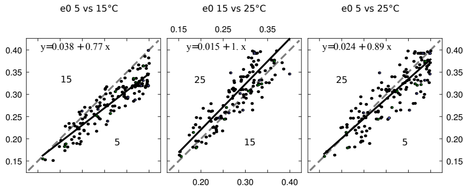
Fig. 5. Correlations between efficiencies at 5, 15, and 25°C from behavioural parameter sets in the one initial quality, flexible decomposer efficiency model. Solid line: linear regression of data. Broken line: 1:1 line.
