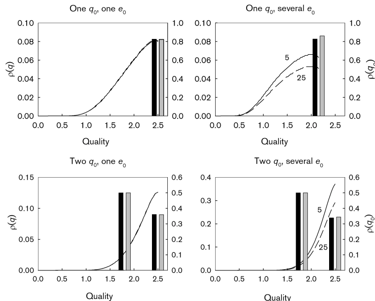
Fig. 6. Distributions of qualities for combinations of one or two initial qualities and fixed or flexible decomposer efficiency ( e_0 ) when 12% carbon has been lost for sample incubated at 5 or 25°C. Solid lines and black bars are for samples at 5°C. Dashed lines and grey bars are for samples at 25°C. The bars have been shifted slightly leftwards and rightwards from their value to visually separate them. Bars show the amount of carbon that has not been used by decomposers so far (remaining at the initial qualities). The lines show the distributions of carbon that the decomposers have converted into new qualities. With flexible decomposer efficiency, more carbon has been converted (lines) and less remains at the initial quality (bar). With two initial qualities the losses have essentially only occurred from the highest quality.
