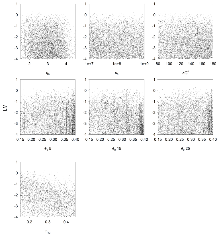
Fig. 4. Dotty plots for the one initial quality, flexible decomposer efficiency. Each dot represents one model run. The likelihood measure, LM, or “goodness of fit”, is plotted against parameter values. The x-scales cover the allowed ranges of the parameters. Parameter sets resulting in a LM > 0 where used in ensemble simulation runs. Only simulations with LM > -4 are shown.
