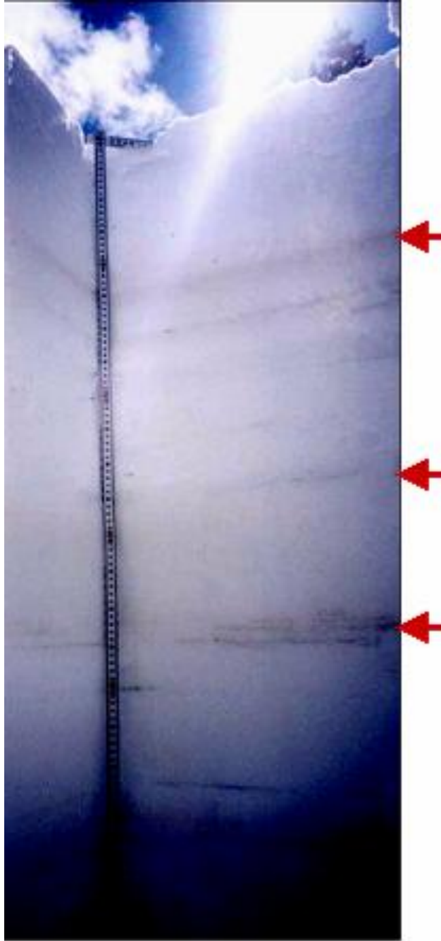
Supplemental Figure 1. Image of distinct dust layers in the snowpack of the San Juan Mountains. Dust layers that were sampled for geochemical analysis in this study are indicated by red arrows. Dust samples were collected in the Senator Beck Basin during the winter of (Photo by Corey Lawrence).
