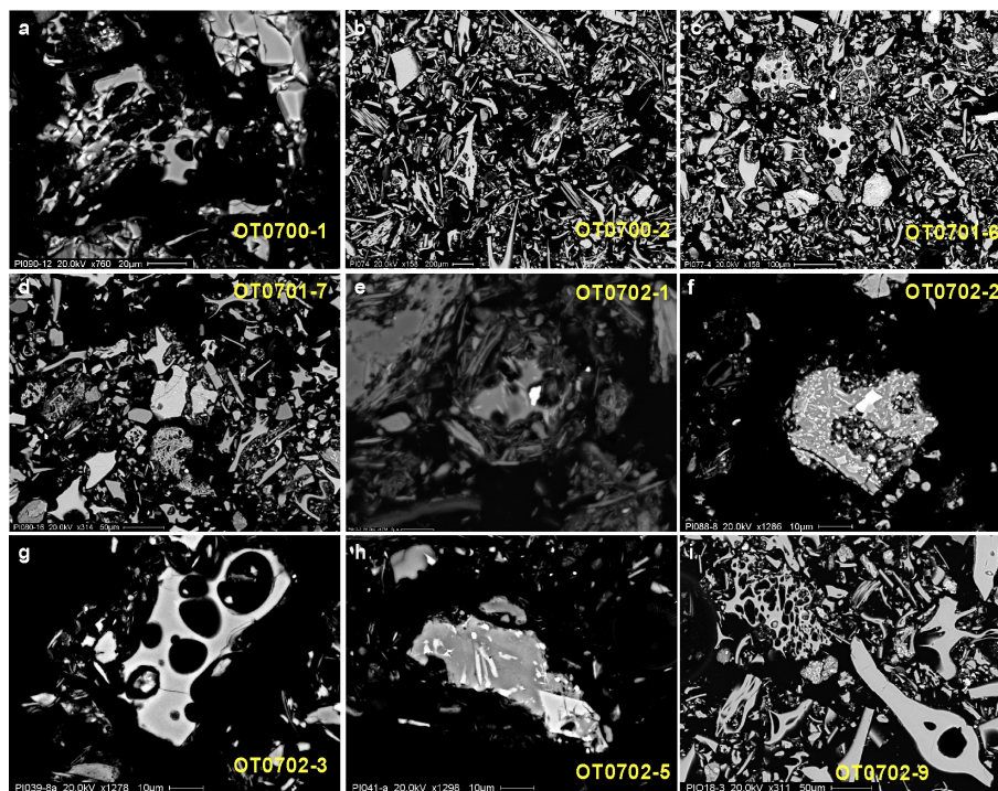
Fig. 4. SEM photographs of volcanic fragments from selected tephra layers and cryptotephra. (a) Y-3 tephra layer in core Co1200; (b) Cl/Y-5 tephra layer from core Co1200; (c) C-20 cryptotephra in core Co1201; (d) X-5 tephra layer in core Co1201; (e) AD 472 cryptotephra in core Co1202; (f) FL cryptotephra in Co 1202 core; (g) Mercato cryptotephra in Co1202 core; (h) Codola cryptotephra in core Co1202; (i) X-6 tephra layer core Co1202.
