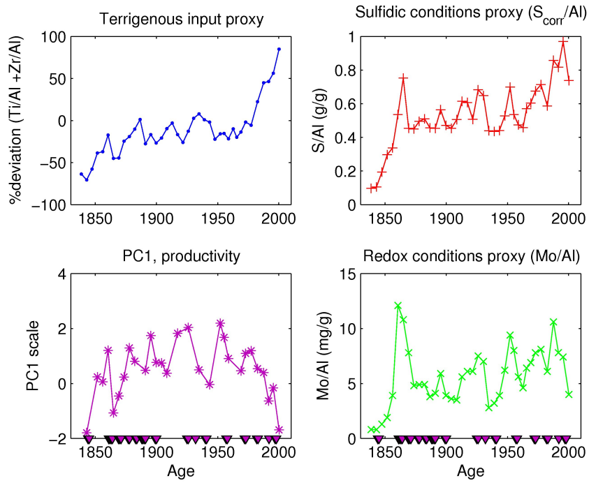
Fig. 1. Comparison of oxygenation and productivity proxies MUC-1B (PC1: principal components summarizing Ba bio , BSi and diatom valve counts). Inverted triangles indicate strong-very strong El Niño events
