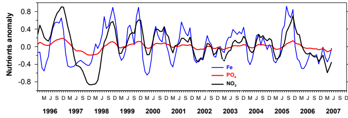
Fig. R1. Anomaly of nutrients in the core of the PFT shift region (140°W-100°W, 10°N-10S) during ENSO cycles.
