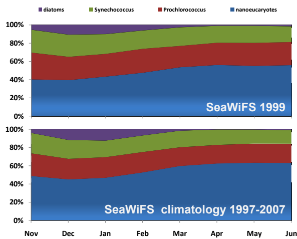
Fig. R2. A comparison of the monthly areal coverage (in percentage) by each PFT obtained from SeaWiFS 1999 year (upper panel) and SeaWiFS climatology between 1997-2007 (bottom panel).
