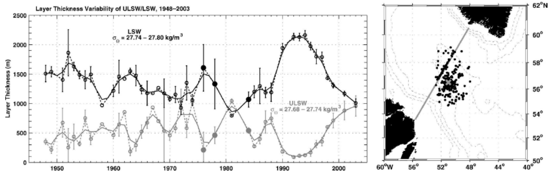
FIG. 12. (left) Time series of layer thickness (m) for classical (black curve) and ULSW (gray curve), given for the period 1948–2003. Open circles indicate the individual mean estimate derived from summer data with vertical bars as the corresponding standard deviation. Filled circles denote estimates solely based on winter data. A 3-yr filter is applied to smooth the time series (solid lines). (right) Location of included Labrador Sea profiles (black dots). The gray line marks the course of WOCE line AR7W; the gray cross is the position of OWS Bravo.
