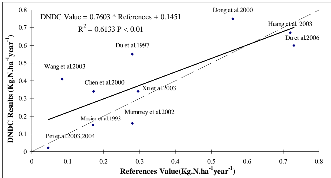
Fig. 2 DNDC results compared with literature reports. Dashed line is 1:1 line (Du et al. 2008 was excluded).
