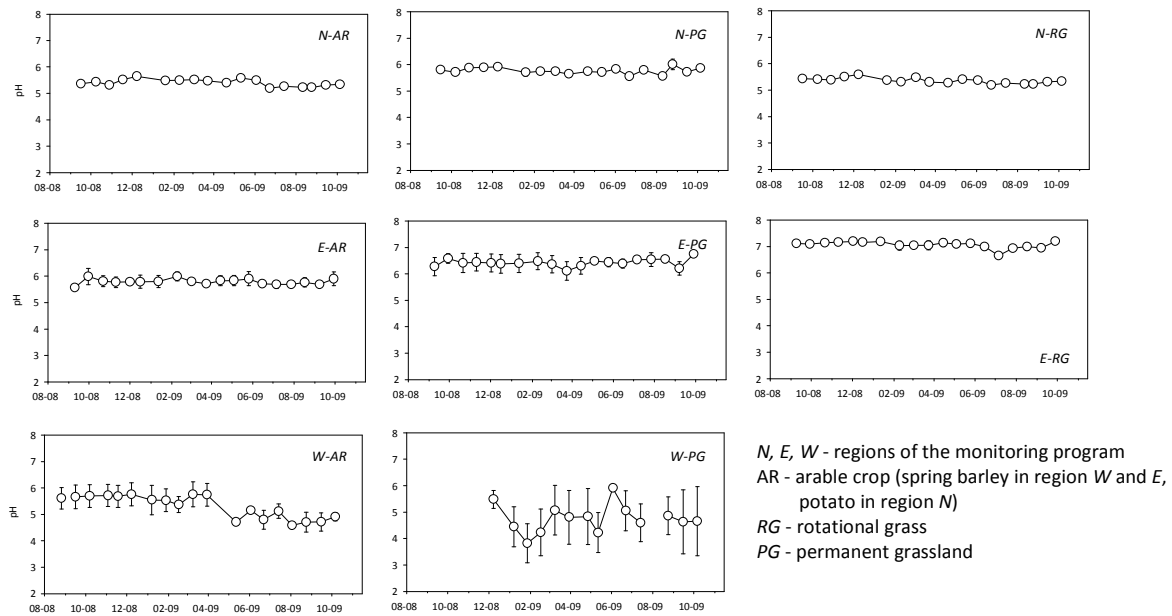
Fig. A1. Seasonal variations in groundwater pH at the eight monitoring sites; Fresh groundwater was sampled from piezometers at the paired sampling points during gas flux measurement campaigns ( n = 3 ; the data shown represent mean \pm standard error). The data set was incomplete due to resource limitations.
