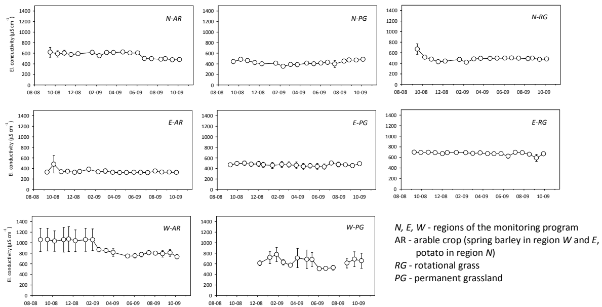
Fig. A2. Seasonal variations in groundwater electrical conductivity at the eight monitoring sites; Fresh groundwater was sampled from piezometers at the paired sampling points during gas flux measurement campaigns ( n = 3 ; the data shown represent mean \pm standard error). The data set was incomplete due to resource limitations.
