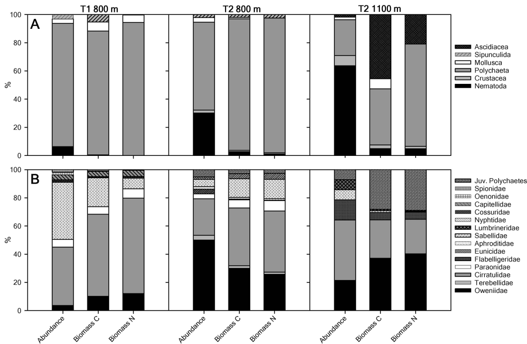
Fig. 3. Relative abundance, biomass C and biomass N of (A) the major macrofaunal taxa and (B) the polychaetes families at stations T1 800 m, T2 800 m and T2 1100 m.
