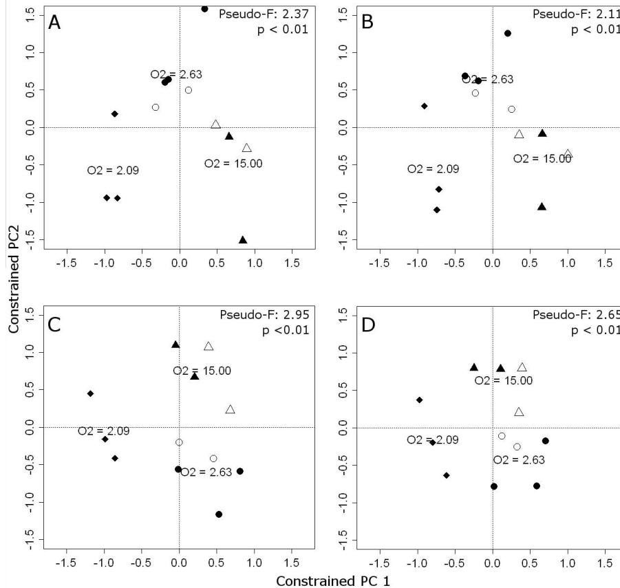
Fig. 7. Constrained ordinations models of macrofaunal assemblage structure, determined by (A) biomass C and (B) biomass N, and the macrofaunal assimilation of (C) _{\text{phyto}} C and (D) _{\text{phyto}} N, at stations T1 800 m (4 day, \blacklozenge ), T2 800 m (4 day \bullet , 7 day \circ ) and T2 1100 m (4 day \blacktriangle , 7 day \triangle ).
