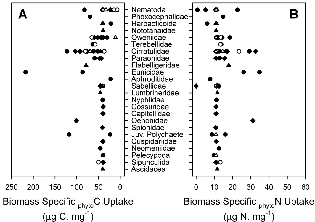
Fig. 6. Biomass specific assimilation of _{\text{phyto}}\text{C} and _{\text{phyto}}\text{N} by individual macrofaunal taxa at stations T1 800 m (4 day, \blacklozenge ), T2 800 m (4 day \bullet , 7 day \circ ) and T2 1100 m (4 day \blacktriangle , 7 day \triangle ).
