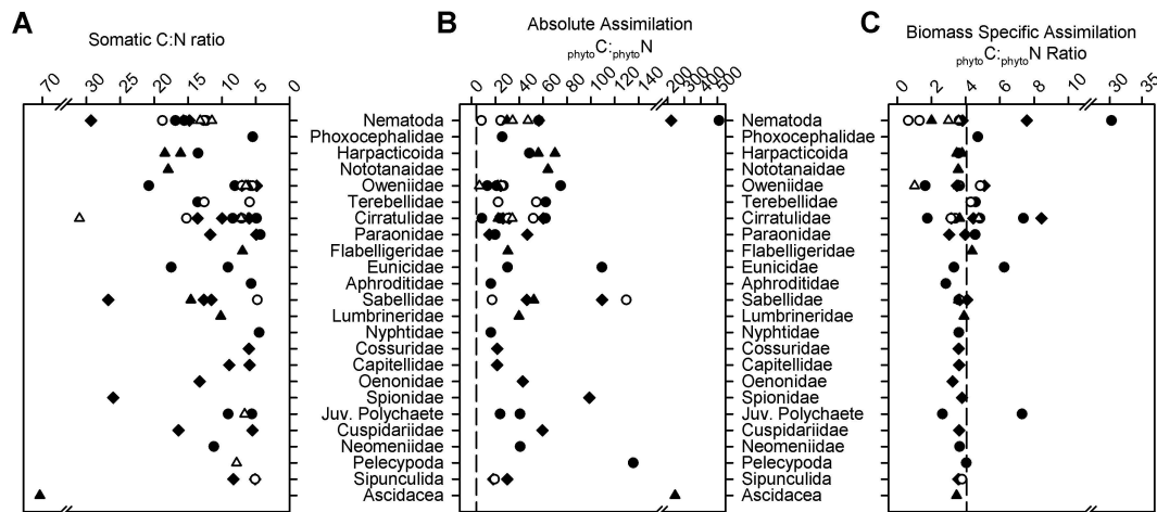
Fig. 8. C:N stoichiometry of the (A) somatic biomass (B) overall assimilation of {}_{\text{phyto}}\text{C} and {}_{\text{phyto}}\text{N} and (C) biomass specific assimilation of {}_{\text{phyto}}\text{C} and {}_{\text{phyto}}\text{N} of individual macrofaunal taxa at stations T1 800 m (4 day \blacklozenge ), T2 800 m (4 day \bullet , 7 day \circ ) and T2 1100 m (4 day \blacktriangle , 7 day \triangle ). Dashed lines represent the phytodetrital C:N ratio as a reference.
