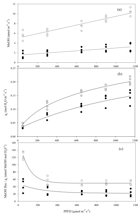
Fig. 1. (a) MeOH emission, (b) stomatal conductance ( g_s ), and (c) MeOH emission normalized for g_s from mature ( n = 4 ; black circles) and immature ( n = 4 ; open circles) L. esculentum over five light levels at constant temperature ( 29 \pm 1^\circ \text{C} ). MeOH emission (slope = 0.0015, t = 4.09 , P = 0.001 for mature; slope = 0.0044, t = 10.52 , P < 0.0001 for immature) and g_s ( F = 112.94 P < 0.0001 R^2 = 0.86 for mature; F = 19.06 P = 0.004 R^2 = 0.96 for immature) significantly increased with PPFD. Normalized MeOH emissions were negatively associated with PPFD (regression coefficient = -0.0006 , z = -5.53 , P < 0.0001 for mature; regression coefficient = -0.0008 , z = -50.20 , P < 0.0001 for immature).
