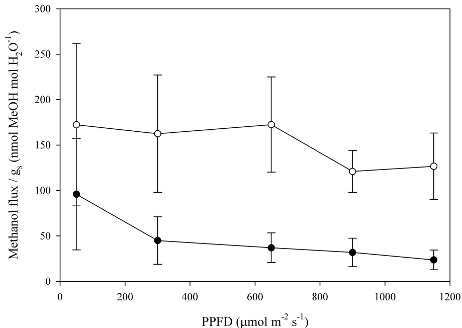
Fig. 2. Average MeOH flux values normalized for stomatal conductance ( g_s ) over five light levels for n=5 mature (black circles) and immature (white circles) L. esculentum (each plant was measured 5x; standard error bars shown). PPFD had no significant effect on MeOH flux for either leaf type ( F = 2.96 ; df = 1, 19 ; P = 0.10 for mature; F = 0.6 ; df = 1, 19 ; P = 0.45 for immature).
