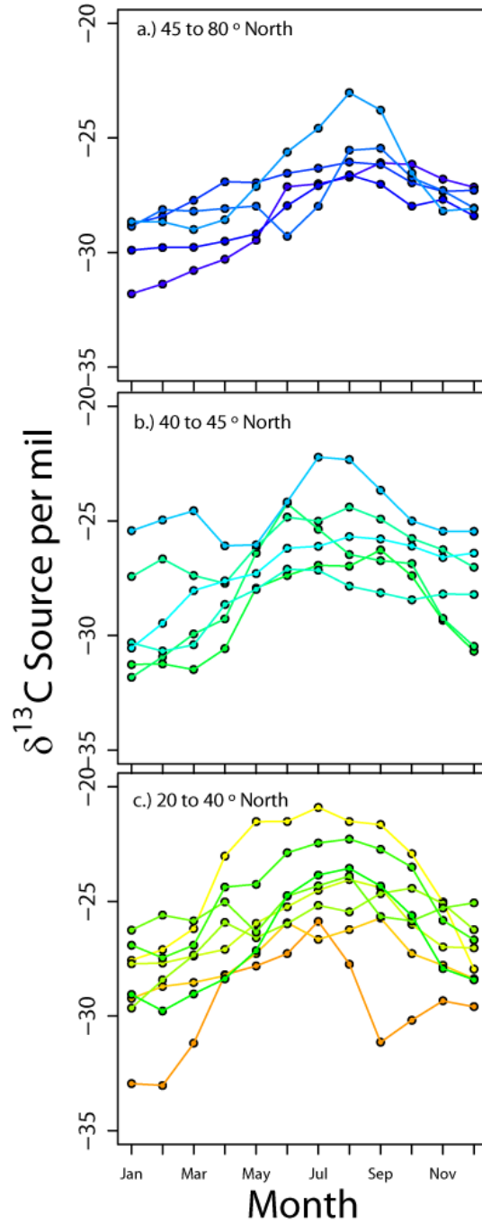
Supplemental Figure 1. Seasonal source values of \delta^{13}\text{C}\text{CO}_2 to the atmosphere grouped by latitude. Sites from 45 to 80°N (a.), 40 to 45°N (b.), and 20 to 40°N (c.) showing the differences in seasonal patterns of source \delta^{13}\text{C}\text{CO}_2 to the atmosphere. Sites are color-coded to correspond with points appearing in Fig. 2A. These are the actual values used to calculate the seasonal anomalies reported in Fig. 2B.
