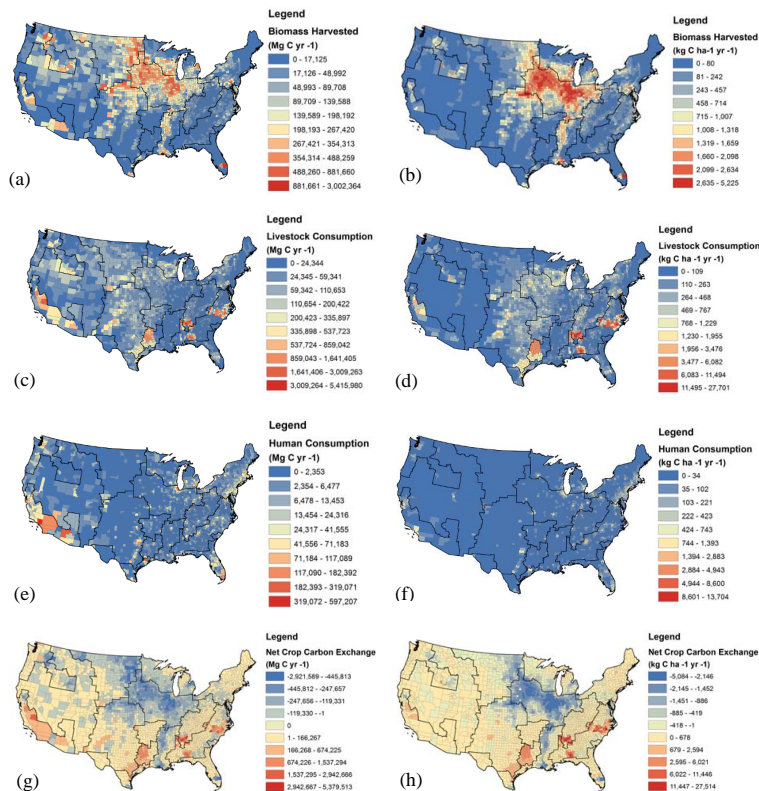
Fig. 4. Harvested biomass, approximate release of biomass carbon from humans and livestock, and the geographic net exchange of crop carbon for 2008. Data are illustrated as mass carbon per county per year ( a, c, e, g ) and as mass carbon per unit area per year ( b, d, f, h ). Harvested biomass ( a, b ) is removed from the field and released as CO 2 by livestock and humans ( c-f ). Net exchange of crop carbon ( g, h ) is the sum of net carbon uptake by crops, net change in soil carbon, and the geographic location of crop carbon release.
