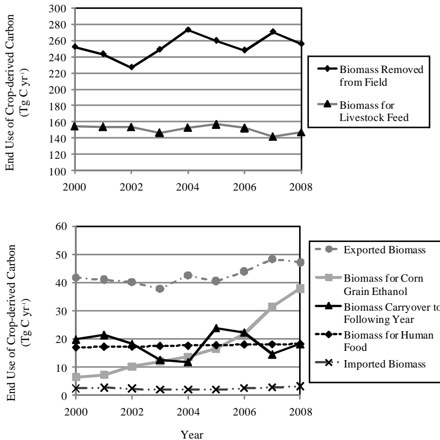
Fig. 2. Components of the US crop carbon budget from 2000 to 2008. Some components of the US crop carbon budget are shown here to illustrate where predominant changes in the budget have occurred between 2000 and 2008. See Table 3 for all components.
