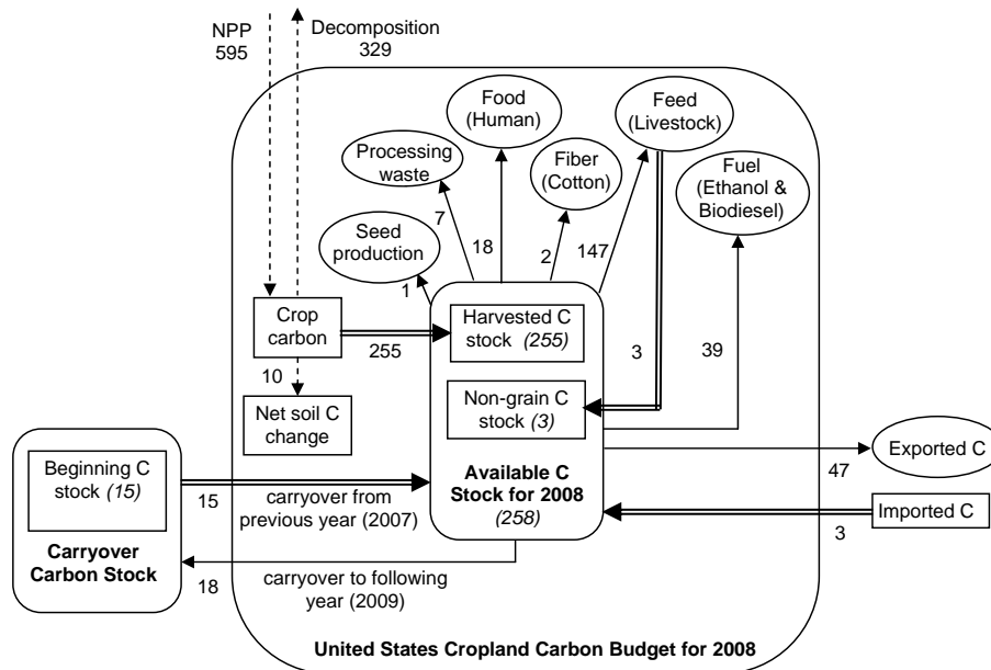
Fig. 1. Cropland carbon budget for the contiguous US. This budget represents the movement of annual crop carbon into, out of, and within the US for the year 2008. Double arrows represent inputs to the annual crop carbon stock that are available for food, feed, fiber, and fuel; single arrows represent flows of carbon that lessen the available crop carbon stock; dashed arrows represent initial photosynthetic production of crop carbon and estimated net soil carbon accumulation. Ellipses represent end uses of crop carbon. All units are in \text{Tg C yr}^{-1} .
