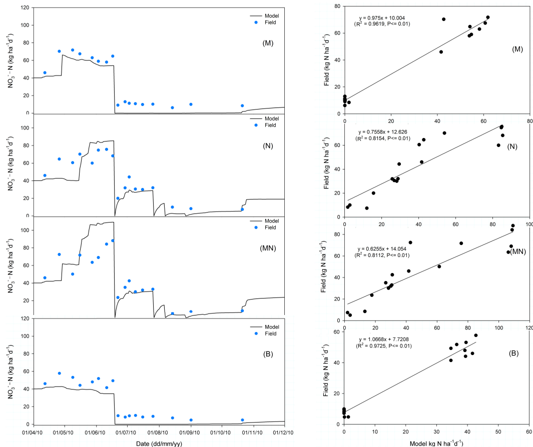
Fig. 1. Fig.1. Comparison of observed and modeled the nitrate (NO 3 - ) for the top 10 cm of the soil profile in summer maize fields
