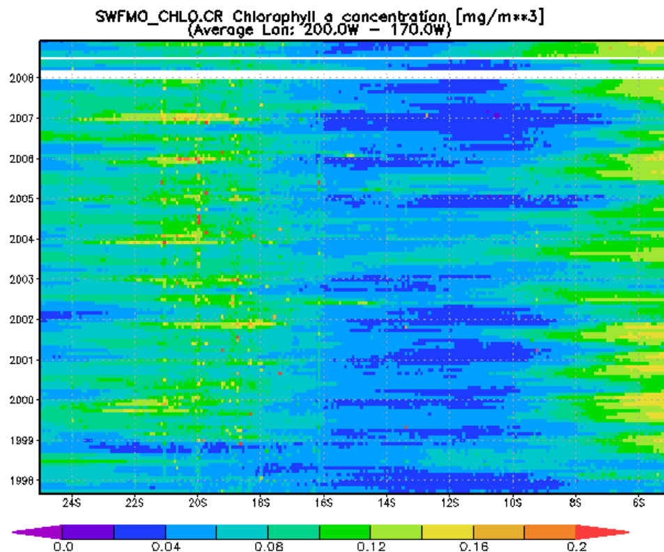
Fig. 1. Monthly time series of chlorophyll concentration
