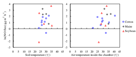
Fig. A2 The relationship between plant N 2 O flux and temperature under dark conditions, based on diurnal observations in the crop fields (2006).
