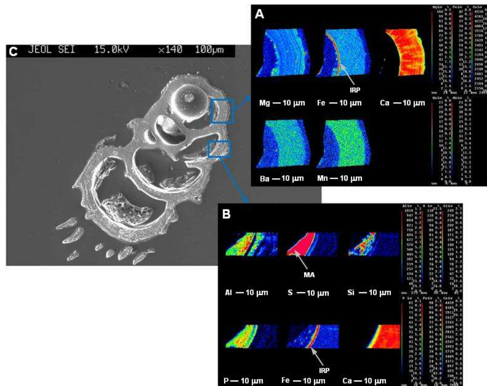
Fig. 2. EMP elemental mappings (A and B) and secondary electron image (C) for an Uvigerina peregrina specimen from 579 m water depth (M77-1-487/MUC-39) on an exposed section of the foraminiferal test. Distribution of Ca, Mg, Fe, Ba, Mn, Al, S, Si and P in the foraminiferal test. All intensity values are expressed in counts per second (cps) as shown in the color bars. IRP: Fe rich phase at inner test surface MA: muddy accumulations inside test chambers.
