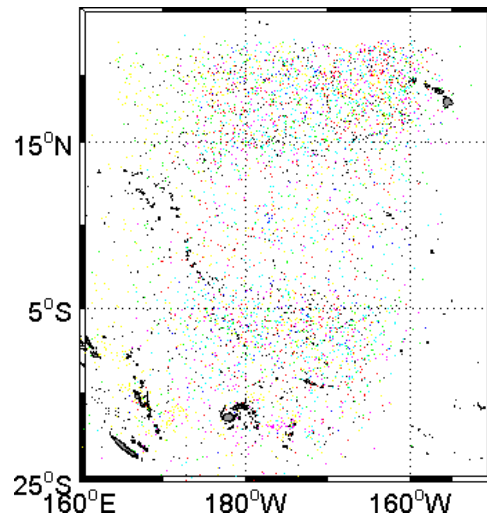
Fig 7C. All boreal summer (austral winter) seasons 1997-2010
