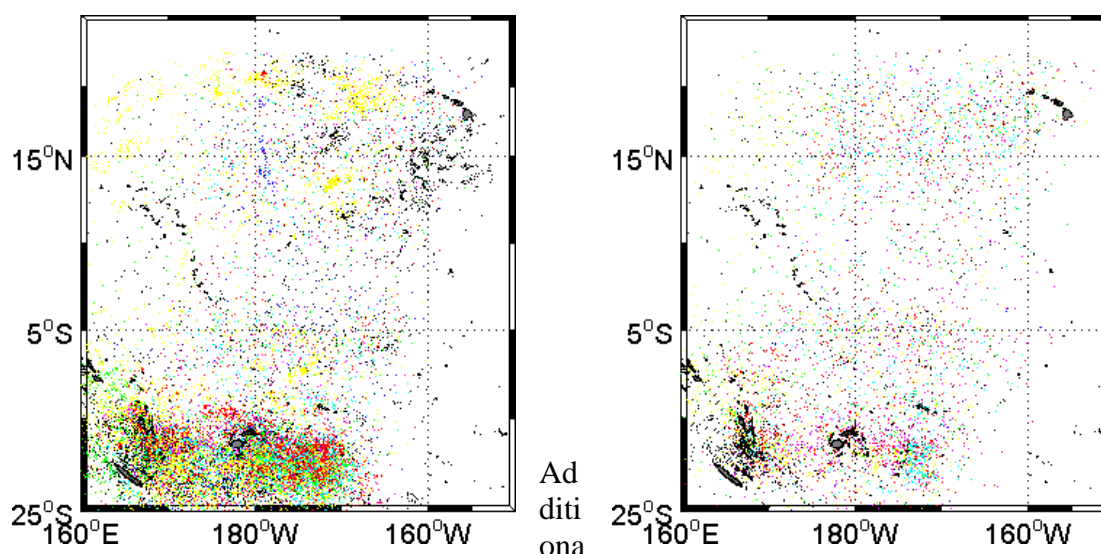
Fig. 7AB (will not be included in the new version). Tricho pixels screened by TRICHOSAT where pixels are represented by a different color per year. A. All summer seasons 1997-2010, B. All inter seasons 1997-2010. Tricho pixels found in 1998 and 1999 years are in yellow and black. Tricho pixels in 2005 are in cyan.
