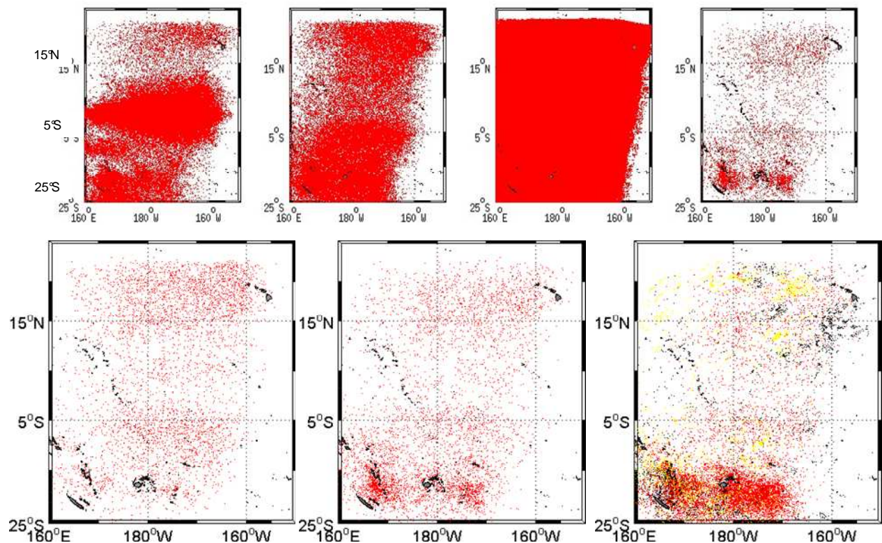
Figure 7 in the new version (old Fig.3)
